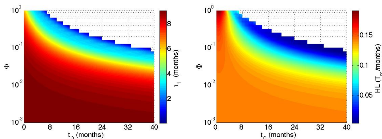
Figure 12. (Left) Heat map for \tau_1(t_0, \Phi) , the time between HBeAb expansion and HBeAg seroclearance, versus the time of HBeAb expansion t_0 and the fraction of core/precure mutations \Phi . The corresponding parameters for wildtype and mutant populations are assumed to be equal and given in Table 1, and s = 6 \text{ mL}/(\text{IU} \times \text{d}) . (Right) Heat map of HL(t_0, \Phi) , the average monthly hepatocyte loss between HBeAb expansion and HBeAg seroclearance due to CTLs killing, versus the time of HBeAb expansion t_0 and the fraction of core/precure mutations \Phi , for \epsilon = 0.7 . Mutations start at time 0.
