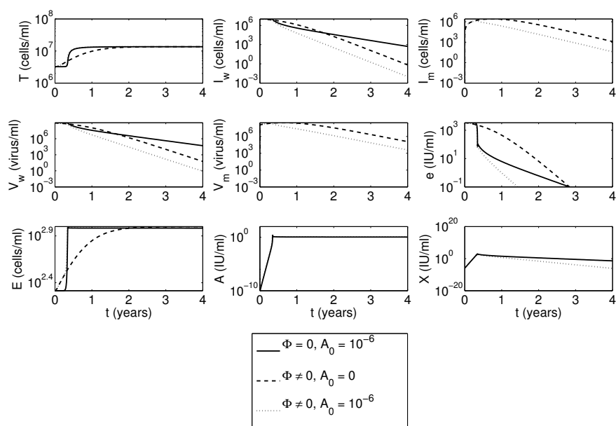
Figure 5. Dynamics of system (3.6) for A_0 = 10^{-6} IU/mL and \Phi = 0 (solid curves); A_0 = 0 IU/mL and \Phi = 0.12 (dashed curves); A_0 = 10^{-6} IU/mL and \Phi = 0.12 (dotted curves). Here, s = 6 mL/(IU \times d), and all other parameters are given in Table 1.
