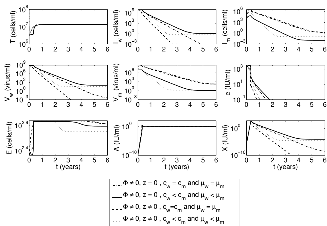
Figure S15. Dynamics of system (S1) when a fraction \Phi = 0.1 of produced virions has core/precore mutations in the absence of transition from I_w to I_m for equal clearance rates of wildtype and mutant virus and wildtype and mutant infected cell (dash-dotted curves), and for increased clearance of mutant virus and mutant infected cells (solid curves); and in the presence of transition from I_w to I_m at rate z = 0.01 with equal clearance rates (dashed) curves, and different clearance rates (dotted curves).
