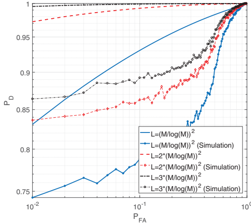
Fig. 3: Approximations and simulation results of P_{FA} versus P_D when the transmitted signal is Gaussian.
