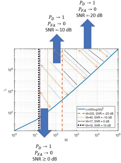
Fig. 2: The convergence of P_D and P_{FA} while L, M go to infinity when the distribution of the transmitted signal is Gaussian.
