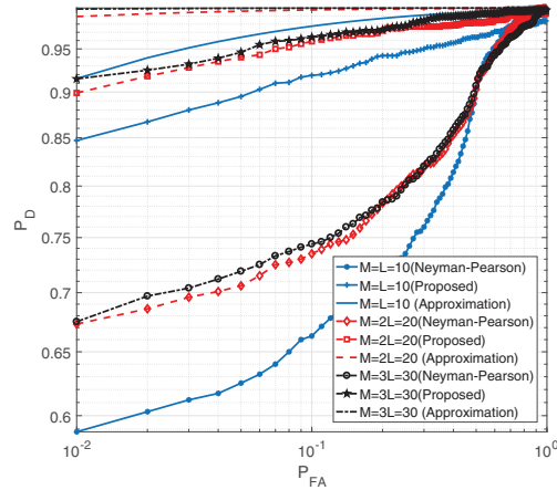
Fig. 4: Approximations and simulation results of the proposed detector and comparison of the results with NP detector when the transmitted signal is non-Gaussian.
