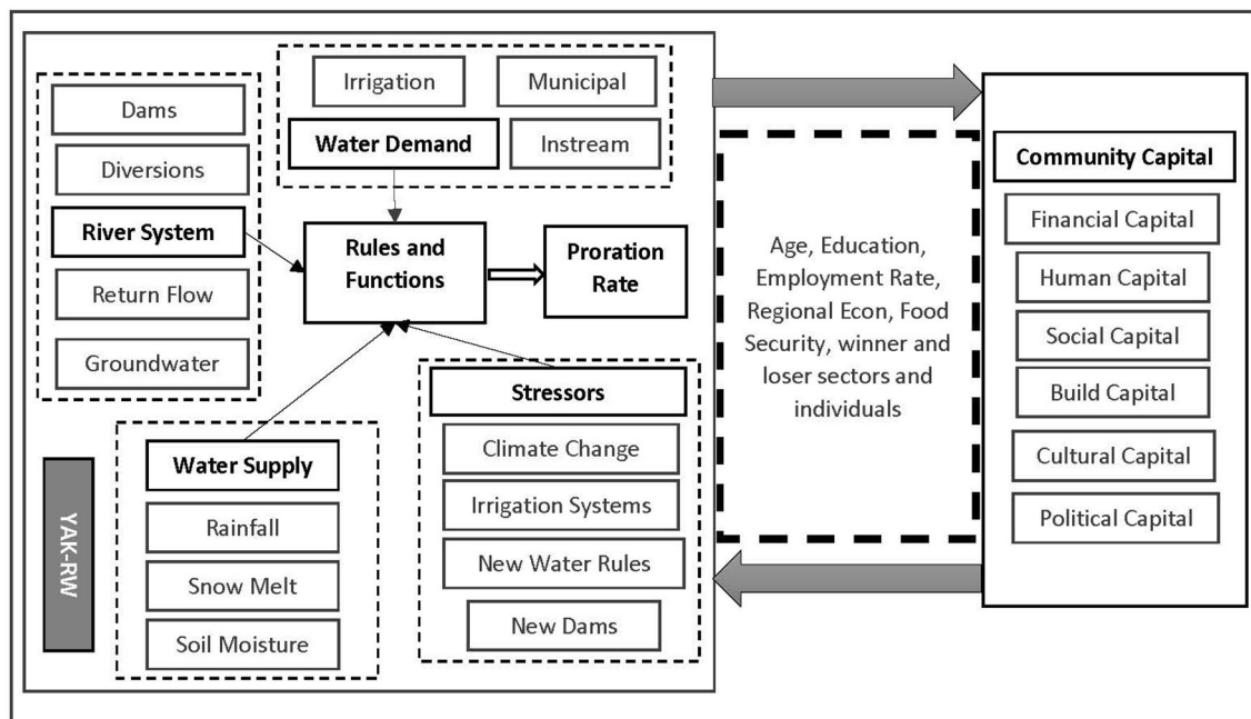
FIGURE 6 | Conceptual map of Yakima River Ware with social components.
