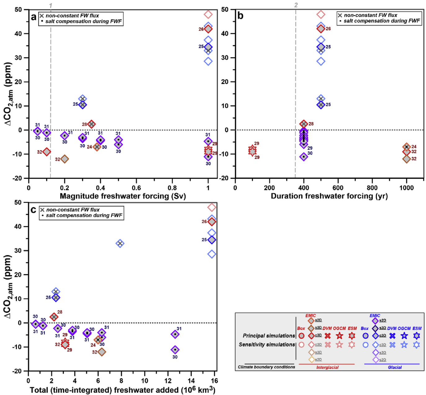
Fig. 10. Simulated \text{CO}_{2,\text{atm}} changes in coupled carbon cycle-climate models forced by FW hosing in the SOc. Simulated \text{CO}_{2,\text{atm}} levels at the end of FWF (which in most cases coincides with the maximum simulated \text{CO}_{2,\text{atm}} change throughout the experiments; cf. pink dots in Fig. 11) as function of the (a) maximum magnitude, (b) duration and (c) total (time-integrated) amount of FW fluxes in the SOc. Symbols are identical to Fig. 3. Symbols with centered black dots highlight simulations that apply global salt compensation during FW hosing. Crosses indicate simulations, which apply non-constant FW fluxes. References and further information on all model simulations are listed in Table 1, Tables S1 and S3. Vertical dashed lines indicate recent estimates of 1) the magnitude of Antarctic FW discharge during meltwater pulse 1A ( \sim 0.11 Sv; Colledge et al., 2014) and 2) the duration of meltwater pulse 1A ( \sim 350 years; Deschamps et al., 2012).
