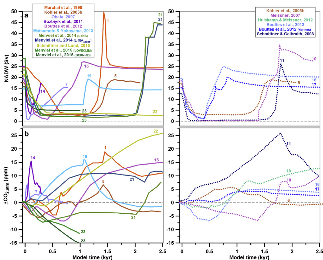
Fig. 7. Timeseries of simulated \text{CO}_{2,\text{atm}} and AMOC change in selected NATI FW hosing experiments. (a) AMOC changes, and (b) variations in simulated \text{CO}_{2,\text{atm}} levels. Solid and dotted lines indicate simulations performed under interglacial and glacial climate boundary conditions, respectively. Numbers refer to Table 1, Tables S1 and S2, which list all details and references of the hosing experiments.
