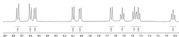
Figure 3: Proton NMR spectrum (400 MHz) of M3 in (\text{CD}_3)_2\text{SO} .
