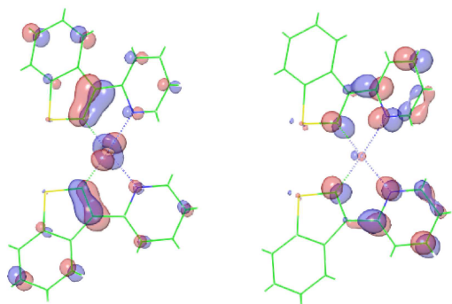
Figure 6. Calculated Hole (left) and Particle (right) wavefunctions for the high oscillator strength calculated electronic transition at 453 nm.
