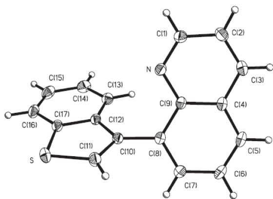
Figure 1. ORTEP of Compound O1 (50% probability thermal ellipsoids). Selected bonds lengths (Å) and angles (°): C7-C8: 1.3781(16); C8-C9: 1.4285(15); C8-C10: 1.4818(15); S-C11: 1.7283(13); S-C17: 1.7376(13); N-C1: 1.3193(15); N-C9: 1.3708(14); C11-S-C17: 91.38(6); C1-N-C9: 117.7(1); C11-C10-C8: 123.4(1); C12-C10-C8: 124.7(1); C7-C8-C10: 120.3(1); C9-C8-C10: 120.70(10)
