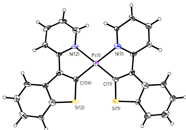
Figure 2. ORTEP of Compound L3 (50% probability thermal ellipsoids). Selected bonds lengths (Å) and angles (°): Pt-N(11): 2.133(7); Pt1-N12: 2.116(7); Pt-C(11): 1.964(9); Pt1-C114: 1.978(9); C11-Pt1-C114: 101.5(4); C11-Pt1-N11: 78.0(3); C114-Pt1-N11: 171.0(4); C11-Pt1-N12: 168.7(3); C114-Pt1-N12: 78.0(3); N11-Pt1-N12: 104.3(3).
