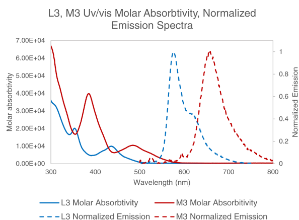
Figure 4: Emission and UV-vis Spectra for the bismetalated species L3 and M3
