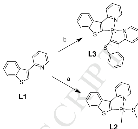
Scheme 1: Reaction of ligand L1 with PtA to form metalated species. a) 2 equiv. of L1 , stirred in toluene 2 h at room temp. followed by heating to 60 for 1 h.; b) L1 with PtA heated at 80 C for 5 h followed by 1 h irradiation with 450 nm light.
