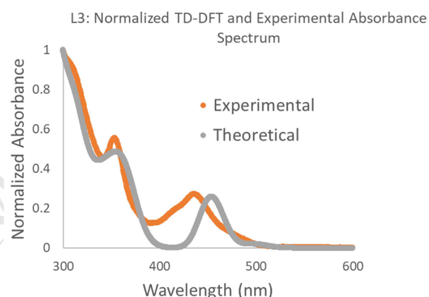
Figure 5. Comparison of experimental and TD-DFT calculated normalized absorbance spectrum. The theoretical absorbance spectrum is visualized by the convolution of the discrete eigen-spectrum with gaussian functions of 25 nm half-width.
