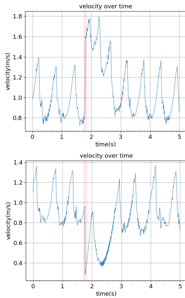
Figure 9. Impact of outside disturbances on the walking speed. Walking speed vs. time is plotted. (top) A 30 kg·m/s impulse is applied to the torso in the walking direction. (bottom) A 40 kg·m/s impulse is applied to the torso opposite to the walking direction.
