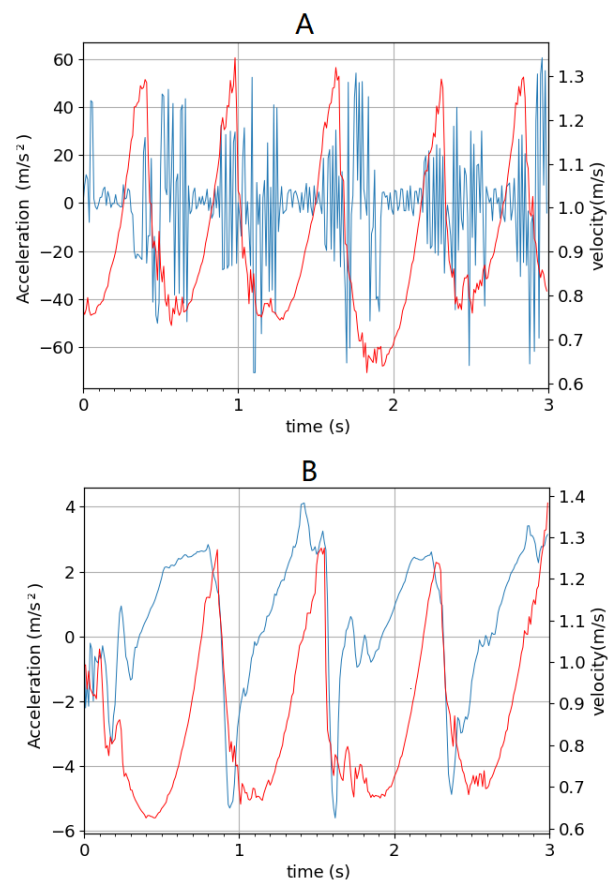
Figure 5. (A) Before and (B) after filtering. The blue line indicates the acceleration; the red line indicates the velocity.
