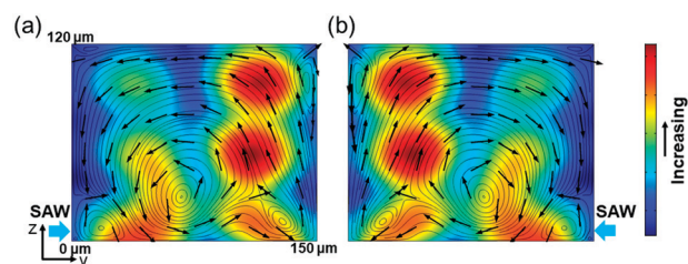
Fig. 2 Simulated acoustic streaming patterns and the distribution of acoustic pressure in the microchannel when the SAW is from either of the IDTs. Red and blue colors indicate high and low magnitudes of acoustic pressure, respectively. The direction of acoustic streaming lines is indicated by the black arrows. (a) The SAW coming from the left side generates a large, counterclockwise vortex in the middle of the channel and some smaller vortices near the edges, whereas (b) the SAW coming from the right side generates a clockwise vortex in the middle of the channel and also some smaller vortices. Moreover, the SAW coming from either side forms a pressure node near the middle of the channel.
