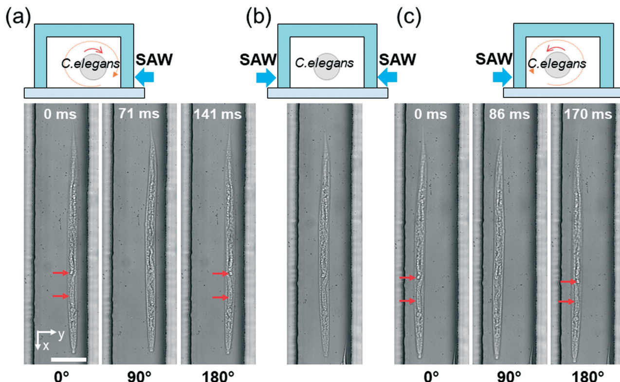
Fig. 4 Rotating C. elegans in opposite directions using SAW. (a) Schematic and image sequences showing that the C. elegans is continuously rotated clockwise when only the right IDT is activated. (b) Schematic and images showing that the C. elegans is focused in the middle of the channel when both of the IDTs are activated. (c) Schematic and images sequences showing that the C. elegans is continuously rotated counterclockwise when only the left IDT is activated. Scale bars: 100 \mu\text{m} . Red arrows point out differences among figures, demonstrating rotation.
