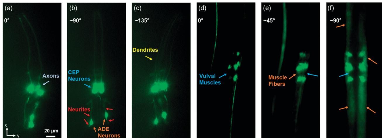
Fig. 7 Examination of the neurons and muscles of the C. elegans from different orientations using our SAW device. (a) Fluorescent image showing the axons between CEP neurons of a L4 stage nematode expressing GFP under the control of the dat-1 promoter [strain BY200, genotype vtIs1 ( pdat-1::GFP; rol-6 )]. (b) After rotating about 90^\circ , all four CEP neurons and neurites around two ADE neurons were clearly displayed in the fluorescent image. (c) After rotating to about 135^\circ , all four dendrites were clearly displayed in the fluorescent image. (d) Fluorescent image showing the side view of the vulval muscles of an adult myo-3::GFP worm [strain RW1596, genotype myo-3(st386); stEx30 ( myo-3p::GFP::myo-3 + rol-6(su1006) )]. (e) After rotating about 45^\circ , all four vulval muscles and some muscle fibers were displayed in the fluorescent image. (f) After rotating to about 90^\circ , all four vulval muscles were shown in the front view, and the muscle fibers were distinguished in the fluorescent image.
