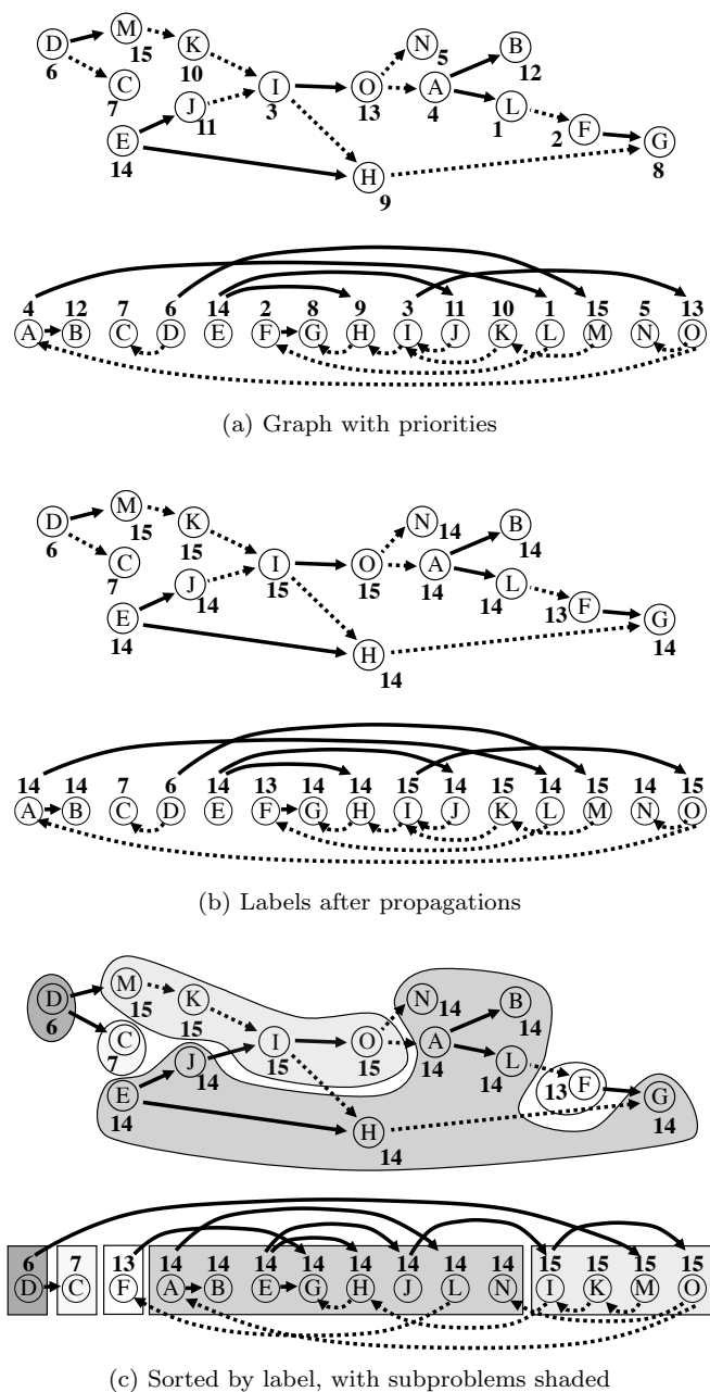
Figure 1: An example of a single level of recursion for Algorithm 1, with d = 2 . Each of the three subfigures shows two equivalent images of the same graph, with the bottom image displaying the current vertex ordering from left to right. Vertices are labeled alphabetically by their initial ordering. Solid arrows represent satisfied edges (i.e., those edges directed to the right in the vertex-ordered graph) and dashed arrows represent violated edges (those edges directed to the left). The number over each vertex is either its random priority (in 1a) or its label (in 1b and 1c).
