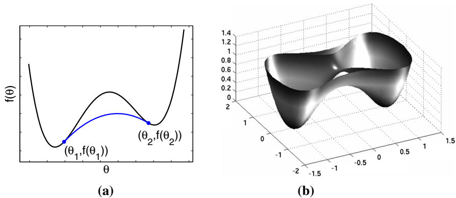
Fig. 2 a The graph of f^{\text{qc}}(\theta) for the example; b relaxed energy QW(F) restricted to diagonal 2 \times 2 matrices F in the (F_{11}, F_{22}) -plane
