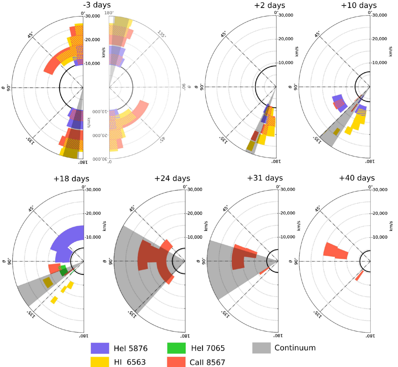
Figure 8. Polar plots of SN 2011hs from -3 to +40 d with respect to V -band maximum light. The P.A. of He I, H\alpha , and Ca II are shown as a function of radial velocity. The velocity of Fe II \lambda 5169 (proxy for photospheric velocity) is shown in black. The hatched areas represent the overlap between elements. The continuum P.A. is shown in grey. It should be noted that the apparent symmetry seen at -3 d is a consequence of the nature of the Stokes parameters being quasi-vectors. The upper and lower arcs are joined at the 0^\circ – 180^\circ boundary, as shown by the faded addition of the rotated diagram of the -3 d plot.
