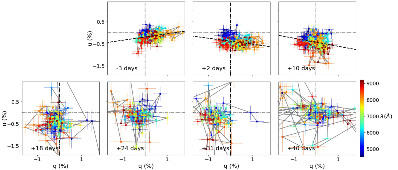
Figure 9. Stokes q - u planes of the ISP corrected data of SN 2011hs from -3 to 40 d after V-band maximum. The data were binned to 15 \text{ \AA} and the colour scale represents wavelength. The dominant axes of epochs 1–3 are shown as the dashed black line, and were calculated using ODR.
