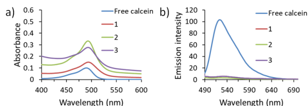
Figure 2. Absorption (a) and emission spectra (b) of free calcein and encapsulated calcein in polymer assemblies.
