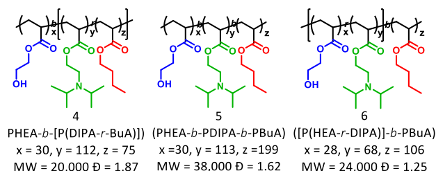
Scheme 4. The structures of tri-component polymers 4–6 .
