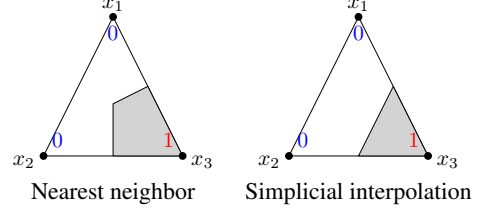
Figure 1: Comparison of nearest neighbor and simplicial interpolation. Consider three labeled examples from \mathbb{R}^2 \times \{0, 1\} : (x_1, 0) , (x_2, 0) , (x_3, 1) . Depicted in gray are the regions (within \text{conv}(x_1, x_2, x_3) ) on which the nearest neighbor classifier and simplicial interpolation classifier predict 1.
