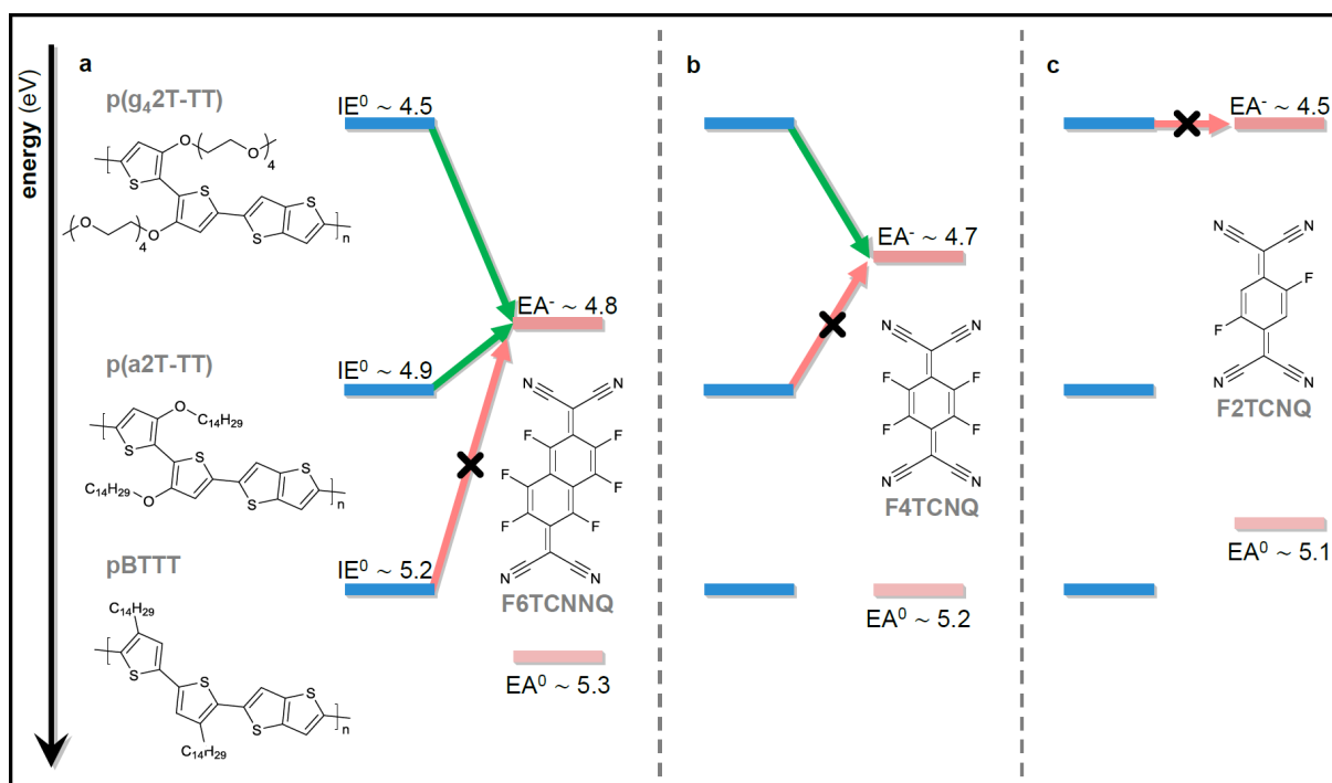
Fig. 2 | Energy diagram summarising the formation of dopant dianions. Doping of p(g 4 2T-TT), p(a 2 T-TT) and pBTTT with a , F6TCNNQ, b , F4TCNQ, and c , F2TCNQ; IE⁰ of the polymers as well as EA⁰ and EA⁻ of the dopants were measured with cyclic voltammetry (CV) (Supplementary Figs. 5 and 6). Green (red) arrows indicate where electron transfer from the polymer to the dopant anion is observed (absent).
