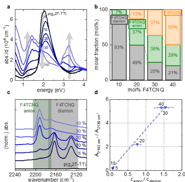
Fig. 3 | Amount of neutral, anionic and dianionic F4TCNQ in doped p(g 4 2T-TT) films.
