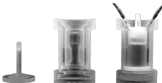
FIG. 5. Sucker core mold insert for bioinspired cup (left) and two-part sucker skin mold for flat bottom sucker shown empty (center) and with completed sucker (right).
