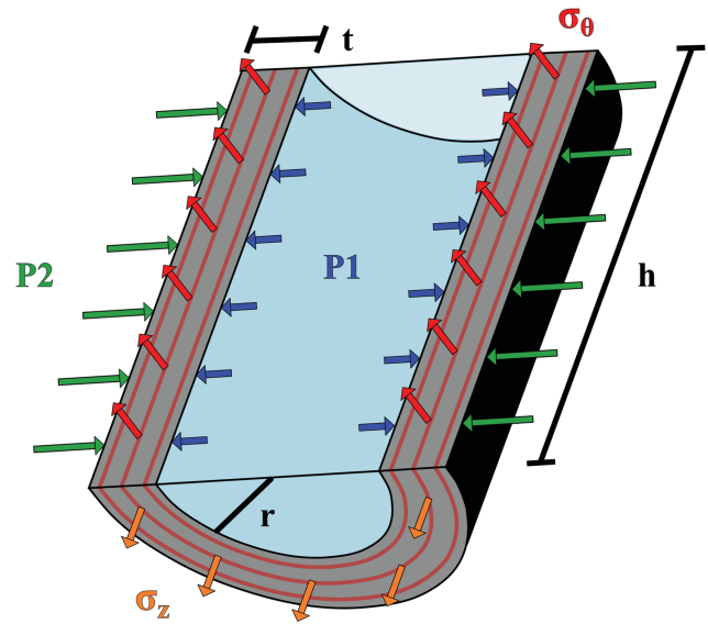
FIG. 11. Cylindrical pressure vessel bisected by two normal planes coincident with and perpendicular to the axis of the cylinder, respectively. Red lines represent DEA layers that compress radially when actuated to create the longitudinal stress \sigma_z (orange arrows) parallel to the cylinder's axis and the tangential stress \sigma_\theta (red arrows) perpendicular to the bisecting plane coincident with the cylinder's axis. A force balance can be applied to each of the bisecting planes to calculate the pressure differential between P_1 (blue arrows) and P_2 (green arrows) in terms of \sigma_z and \sigma_\theta . Color images are available online.
