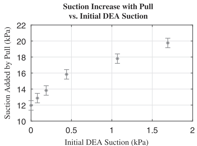
FIG. 20. Increase in suction pressure during pull-off test ( P_{\max} - P_{\text{DEA}} ) versus initial DEA suction ( P_{\text{DEA}} ). Activating the DEA has a greater impact on overall suction than simply adding its own generated pressure during pull-off testing. P_{\max} is represented by each star in Figure 19, while P_{\text{DEA}} is the difference between the measured pressure differentials before and after DEA activation, shown in Figure 18. The error bars shown are for the standard deviation between data sets.
