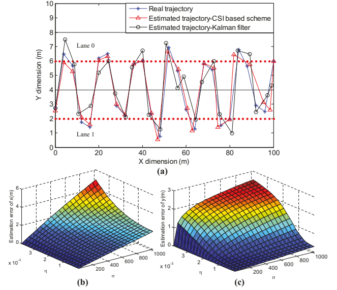
Fig. 4. (a) Trajectory estimation, (b) estimation errors of x -dimension, (c) estimation errors of y -dimension.
