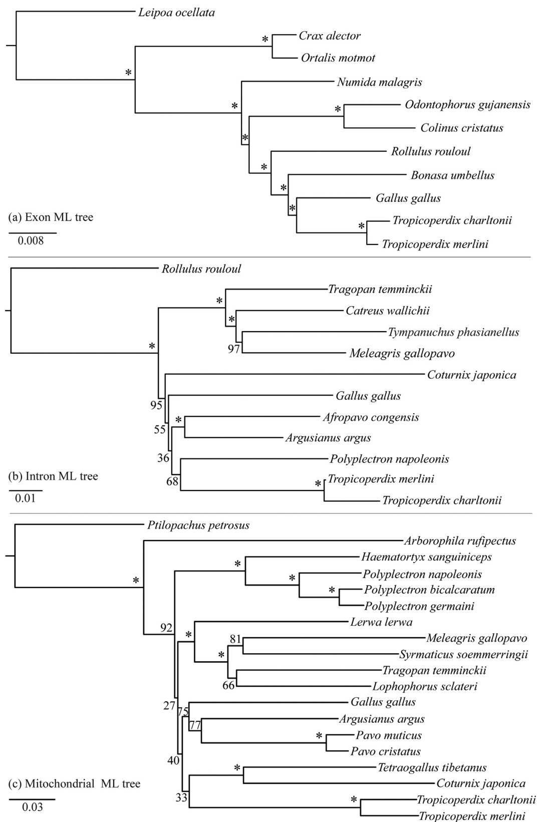
Fig. 4. ML trees from different data types obtained by mapping to Gallus gallus : exons (a), introns (b), and the mitochondrial genome (c). Nodes with 100% bootstrap support are indicated with asterisks *.
