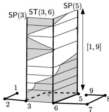
■ Figure 3 A free space diagram \text{FSD}_\delta(P, G) with strips and spines.
