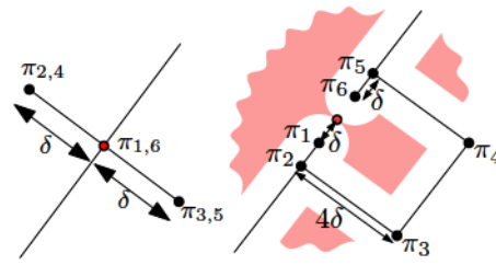
■ Figure 5 Pinhole gadgets \pi for F_C(P, \delta) (left) and \bar{H}_C(P, \delta) (right). The pinhole is shown in red.
