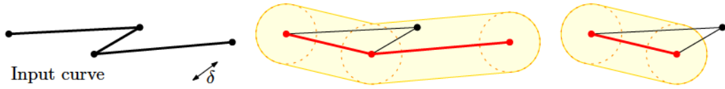
■ Figure 1 For a target distance \delta , the red curve (middle) is a global simplification of the input curve (left), but it is not a local simplification, since the first shortcut does not closely represent its corresponding curve section (right). The example works for both Hausdorff and Fréchet distance.
