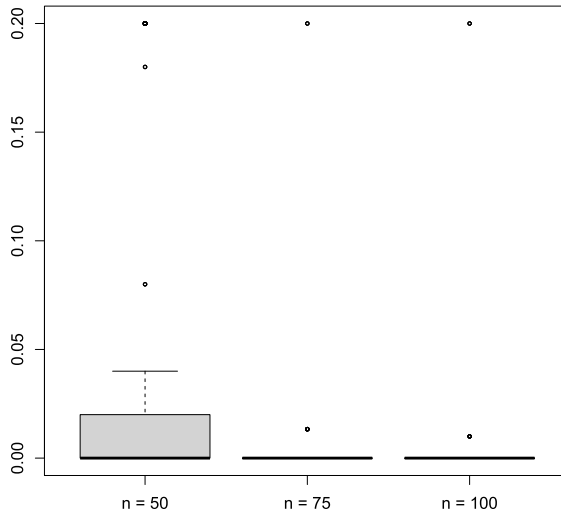
Figure 1. Fraction of misclassified nodes based on 100 simulated data sets with n = 50 , n = 75 , and n = 100 nodes and K = 5 blocks of equal size, where the model is estimated by Bayesian methods.
