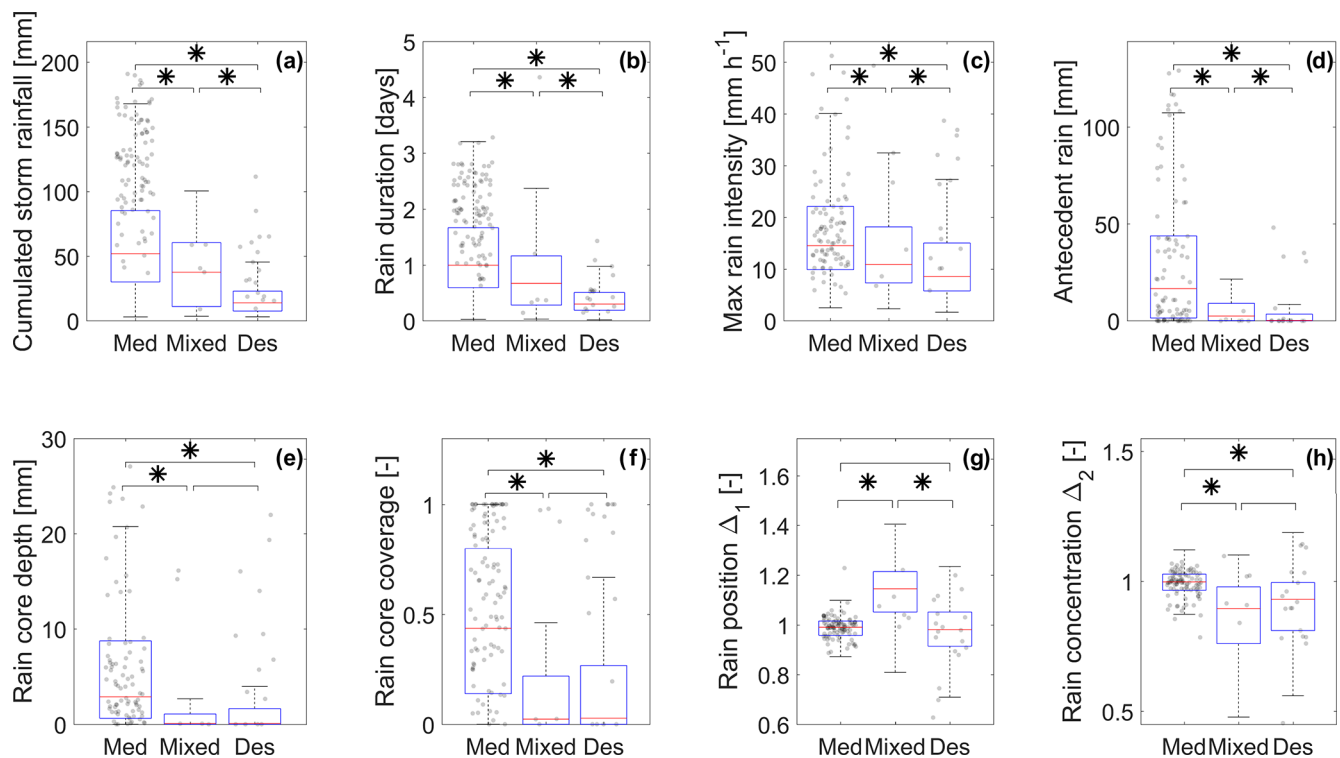
Figure 4. Boxplots showing the distribution of event rainfall properties in the three climate classes. The asterisk describes distributions with a statistically different median (Wilcoxon test, p value < 0.05). Black dots represent floods with more than 5 years of return period; outliers are not presented.
