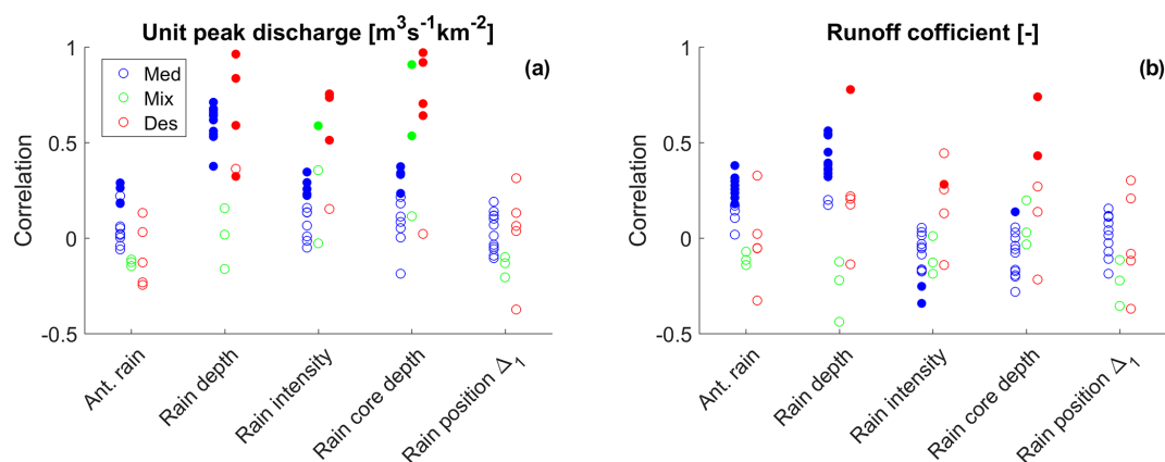
Figure 7. Correlations of the unit peak discharge and runoff coefficient for each basin with more than 15 floods. Each dot represents one basin and filled dots indicate statistically significant correlations (Wilcoxon test, p value < 0.05 ).
