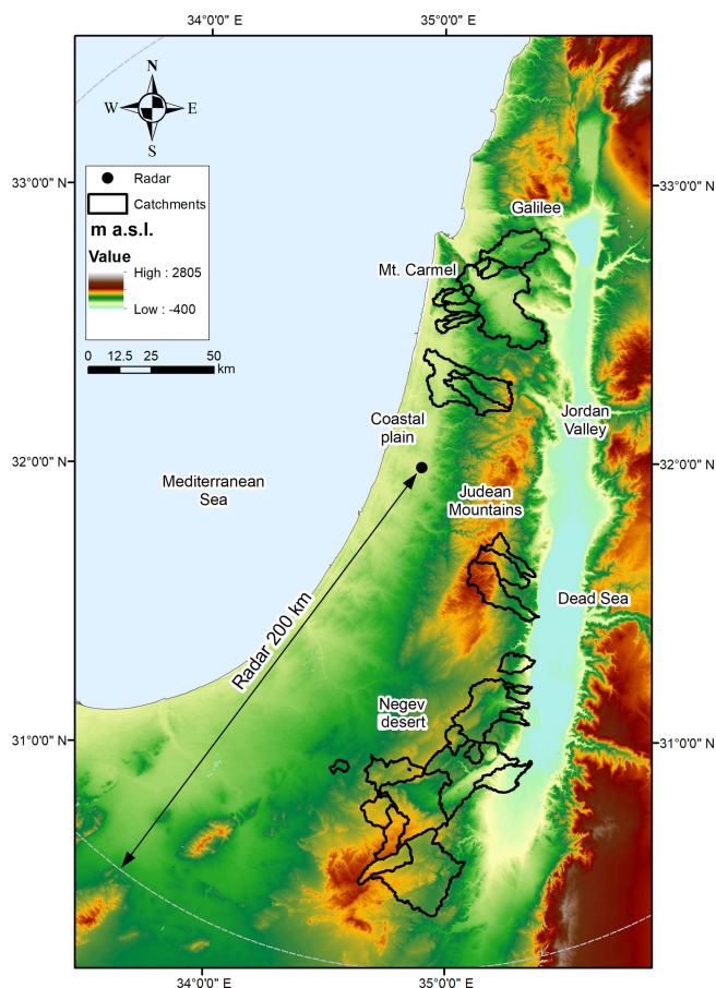
Figure 2. Study area and the outline of the catchments analyzed.
