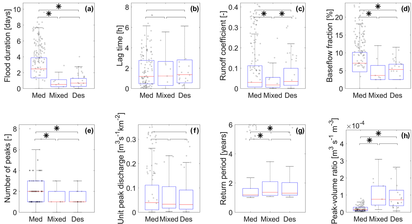
Figure 5. Boxplots showing the distribution of event runoff properties in the three climate classes. The asterisk describes distributions with a different median (Wilcoxon test, p value < 0.05). Black dots represent floods with more than 5 years of return period; outliers are not presented.
