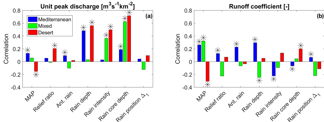
Figure 6. Pearson correlations between unit peak discharge and other parameters among floods of different regions. The asterisks indicate statistically significant correlations (Wilcoxon test, p value < 0.05).
