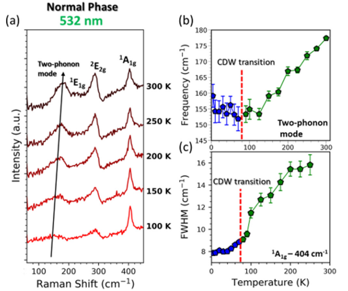
FIG. 3. (a) Temperature-dependent Raman spectra of the higher frequency modes in the metallic phase using 532 nm laser excitation. (b) Evolution of the two-phonon mode frequencies with temperature in and out of the CDW phase as a function of temperature. Below T_{\text{CDW}} , the mode freezes in response to the CDW modulation while softens at higher temperatures. (c) FWHM of the high wave number optical mode at 1A_{1g} 404 cm ^{-1} showing similar broadening response at higher temperatures whereas the phonon linewidth remains consistent in the CDW regime.
