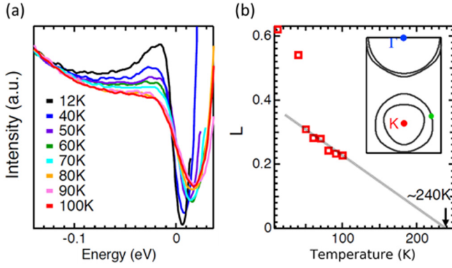
FIG. 4. (a) Fermi-function-divided EDCs with increasing temperature through the T_{\text{CDW}} . (b) The green dot on the schematic plot of the Fermi surface in the inset shows the momentum location of the Fermi-function-divided EDCs in (a). Temperature dependence of the spectral weight at the chemical potential. Extrapolation of L(T) = 1 - \frac{I(T, \omega=0)}{I(T, \omega=\omega_{\text{peak}})} to zero provides an estimate of T^* \sim 240 K, which is much higher than T_{\text{CDW}} .
