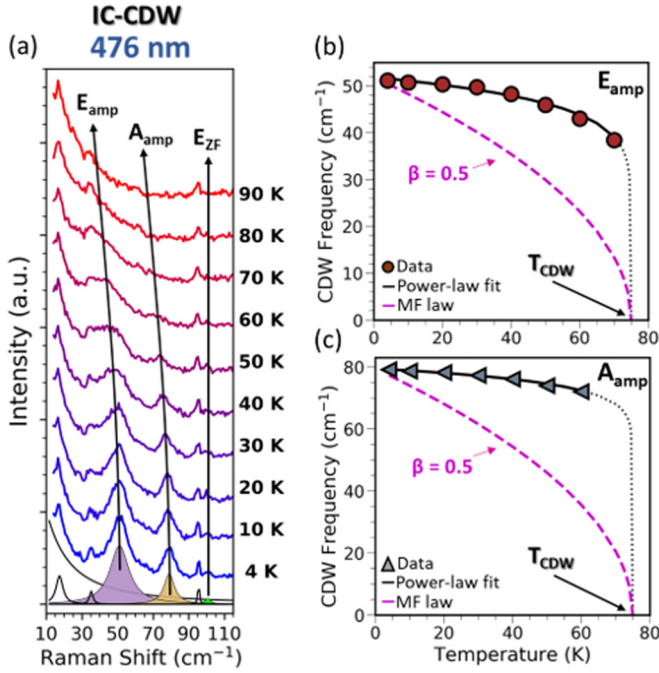
FIG. 2. (a) Temperature-dependent Raman spectra of the CDW modes E_{\text{amp}} and A_{\text{amp}} using 476 nm excitation with a sample Lorentzian fit shown for the data at 4 K. (b) Frequency of CDW mode E_{\text{amp}} extracted from the fits plotted as a function of temperatures. The value of T_{\text{CDW}} is fixed at 75 K (c) Frequency of CDW mode A_{\text{amp}} extracted from the fits plotted as a function of temperature. The value of T_{\text{CDW}} is fixed at 75 K. Dashed magenta line shows a model fit to mean-field theory equation with square-root dependence.
