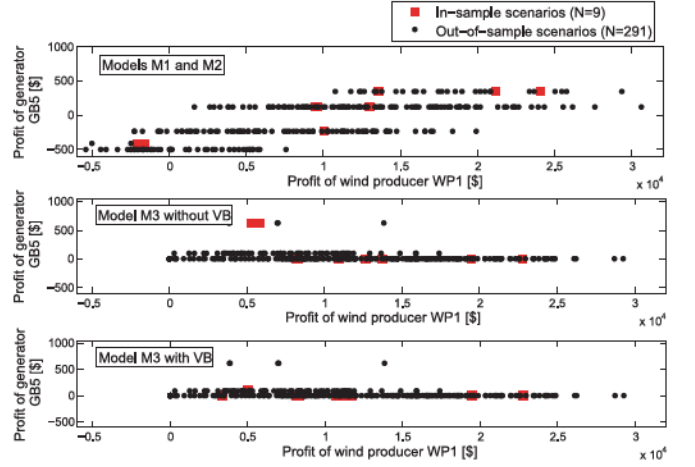
Fig. 3. IEEE two-area RTS case study: Profit of generators GB5 and WP1 in models \mathcal{M}_1 and \mathcal{M}_2 (upper plot), model \mathcal{M}_3 without VB (intermediate plot) and model \mathcal{M}_3 with VB (lower plot) under each in-sample and out-of-sample scenario.
