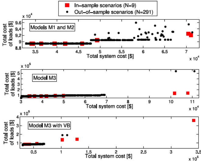
Fig. 4. IEEE two-area RTS case study: Total system cost and total cost of loads in models M1 and M2 (upper plot), model M3 without VB (intermediate plot) and model M3 with VB (lower plot) under each in-sample and out-of-sample scenario.
