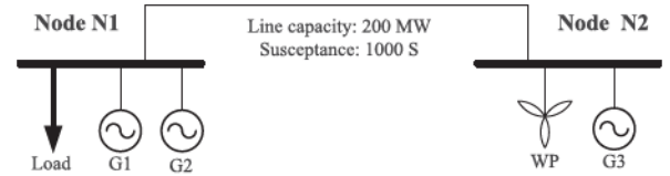
Fig. 1. Network of the illustrative example.
