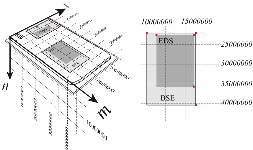
Fig. 7. The grid system applied to thin sections, shown relative to the reference axes (A) or in a horizontal plane (B). The zero point for the grid system along the l - and m -axes is the reference corner. The zero for the n -position is at the top of the rock chip. The grid works in a similar way to the Universal Transverse Mercator (UTM) grid system, with the first position denoting the cm position and decreasing by an order of magnitude in spatial scale with the last position denoting the nanometer position. Different images - from different analytical instruments - can be overlaid on the grid. The position of these images are recorded as ( l , m , n ) coordinates for the corners of parallelograms (shown) or as a center point ( l , m , n ) with radius for circles (not shown).
