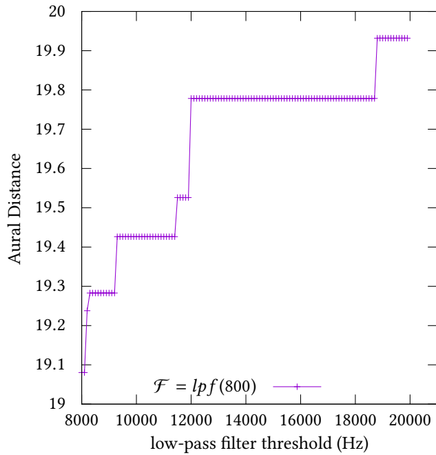
Figure 5. Looking at the portion of a curve from Figure 3 between 8k Hz and 20k Hz, we see the aural distance function is not perfectly convex on the macro scale. In this case, that is because the sample has very few frequencies above the 8k Hz range.
