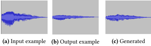
Figure 1. The waveforms (a) and (b) are provided as examples, and DSP-PBE synthesizes a filter that produces (c).
