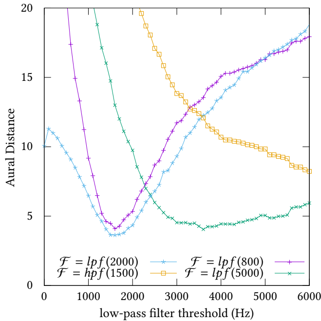
Figure 3. The distance curves showing the convex-like shape of the aural distance function. Each curve is the distance between an input file, and a filter applied to that file - dist(I, \mathcal{F}(I)) .
