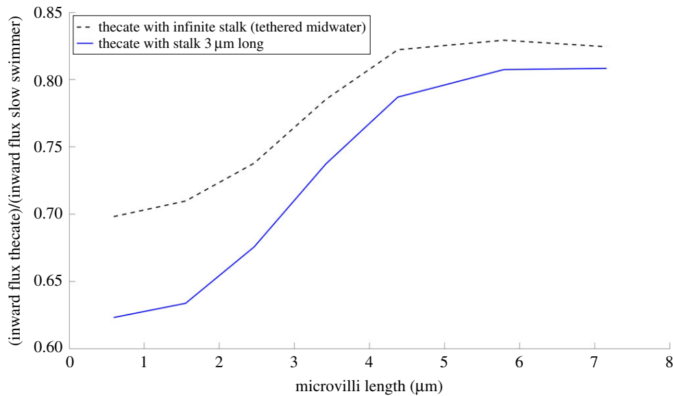
Figure 10. Ratio of inward fluxes to capture zone during a flagellar beat of a thecate cell with stalk length of 3 \mu\text{m} to that of a free-swimming cell as the microvilli length increases (solid blue curve). Also shown is the ratio for cell tethered midwater (infinite stalk length) to a free-swimmer (dashed black curve). (Online version in colour.)
