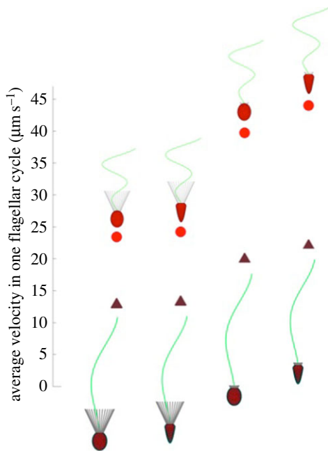
Figure 5. Computed swimming velocities of eight swimmers with two different cell body shapes, two different collar lengths and two different flagellar waveforms. Flagellar arclength is fixed at 27 \mu\text{m} , and the flagellar waveform is varied for each combination. Note that in figure 4, the velocities of the slow swimmer and fast swimmer were nearly equal at this arclength. (Online version in colour.)
