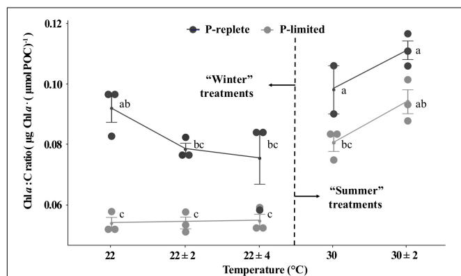
FIGURE 4 | Chl a to C ratios of Trichodesmium GBRTLI101 at five constant and variable temperature treatments and two P conditions (light gray symbols: P-limited culture, 0.2 \mu\text{mol/L} ; dark gray symbols: P-replete culture, 10 \mu\text{mol/L} ) in summer and winter experiments. Values and error bars, respectively, represent the means and the standard deviations of triplicate cell cultures under each treatment. The letters represent the significant differences based on the grouping results of the Tukey multiple comparison among ten temperature \times P treatments.
