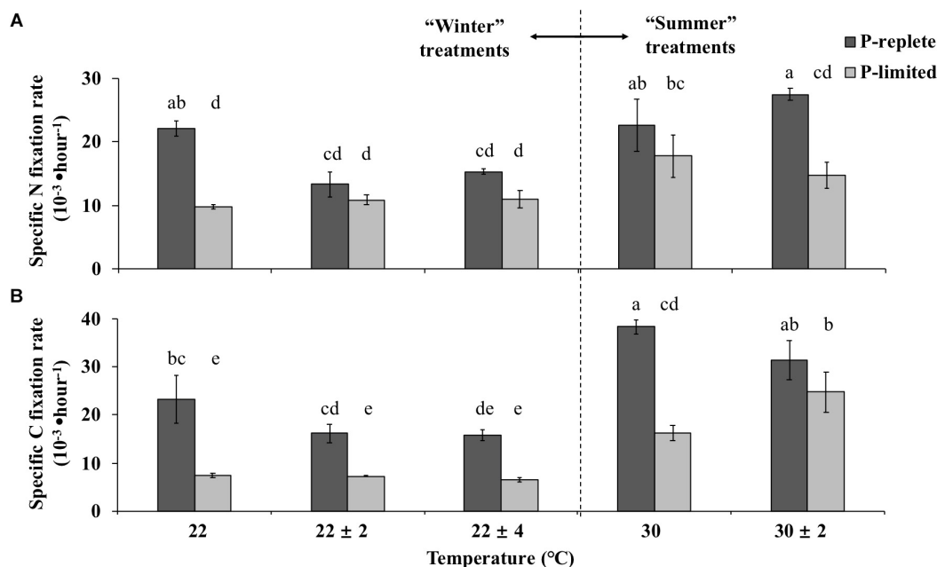
FIGURE 3 | Average (A) nitrogen-specific fixation rates and (B) carbon-specific fixation rates normalized to PON and POC, respectively, of Trichodesmium GBRTL101 in five constant and variable temperature treatments under two P conditions (10 and 0.2 \mu\text{mol/L} ) in summer and winter experiments. Values and error bars, respectively, represent the means and the standard deviations of triplicate cell cultures under each treatment. The letters represent the significant differences based on the grouping results of the Tukey multiple comparison among ten temperature \times P treatments.
