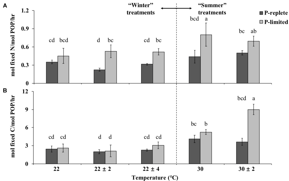
FIGURE 5 | Phosphate Use Efficiency (PUE) for nitrogen (A) and carbon (B) fixation under P-replete and P-limited conditions (10 and 0.2 \mu\text{mol/L} ) in five different constant and variable temperature treatments in summer and winter experiments. Values and error bars, respectively, represent the means and the standard deviations of triplicate cell cultures under each treatment. The letters represent the significant differences based on the grouping results of the Tukey multiple comparison among ten temperature \times P treatments.
