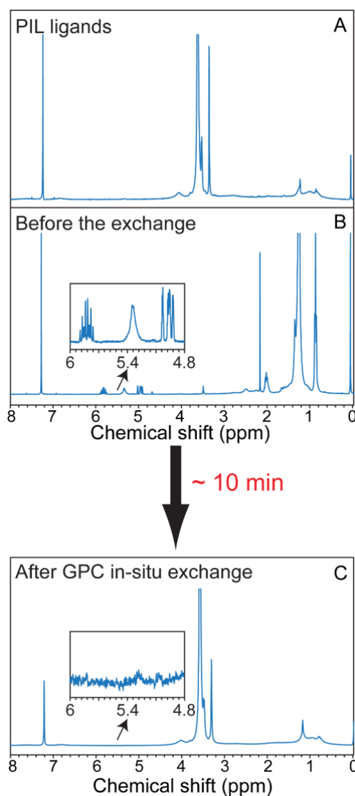
Fig. 5. GPC in situ ligand exchange with MA-PIL macromolecular ligand monitored by ^1\text{H} NMR. (A), spectrum of the pure MA-PIL polymer. (B), spectrum of the oleate-capped CdSe/CdZnS NCs stock solution. (C), in situ exchanged MA-PIL-capped CdSe/CdZnS NCs. Insets expand the olefin resonance region to confirm the completeness of the exchange reaction.
