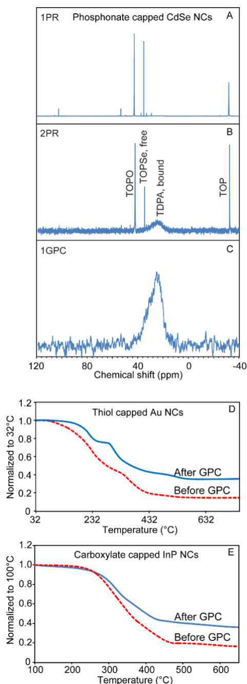
Fig. 1. Purification of NCs with variety of composition and capping ligands. (A)–(C) 31 P NMR of the TDPA-capped CdSe NCs purified by (A) one PR step, (B) two PR steps, and (C) one GPC purification. (D)–(E) TGA curves for the thiol-capped Au NCs (D) and carboxylate-capped InP NCs (E) before (dashed lines) and after (solid lines) the GPC purification.
