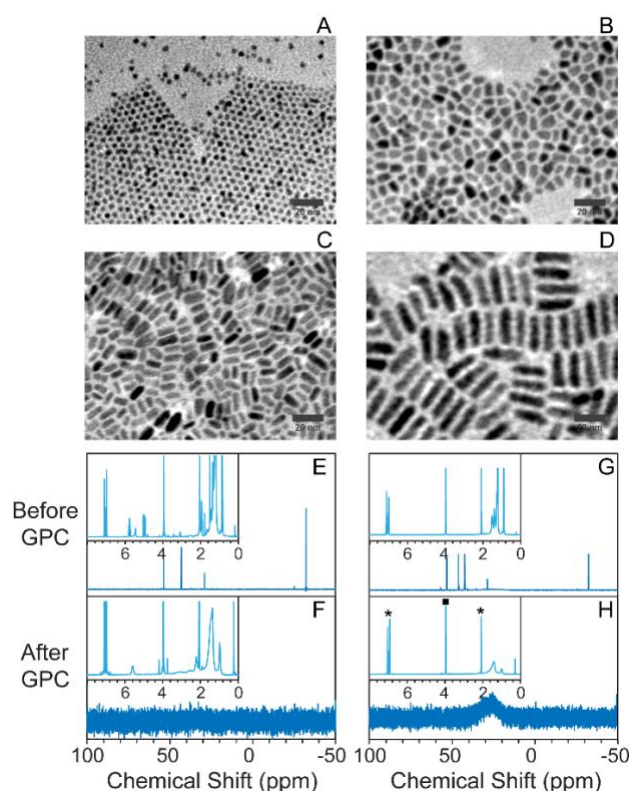
Fig. 2. Purification of CdSe/CdS NCs with variety of morphologies. (A)–(D) TEM images of the NCs in different shapes ranging from spherical NCs to nanorods; from A to D, samples were labelled as CdSe/CdS_NC_1 to CdSe/CdS_NC_4; (E–H) 31 P NMR of the CdSe/CdS_NC_1 (E,F) and CdSe/CdS_NC_2 (G,H) before (E, G) and after (F, H) the GPC purification with 1 H NMR spectra shown as the insets. Asterisks in (H) inset indicate peaks associated with the toluene solvent that are present in each sample. The square indicates the signal from the ferrocene internal standard.
