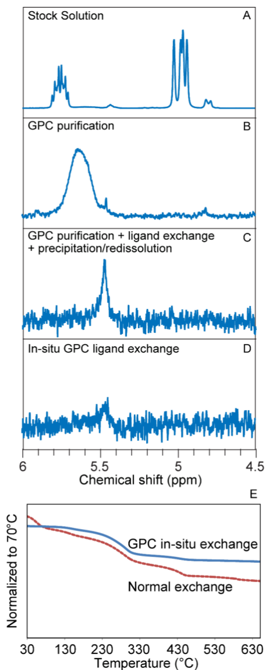
Fig. 4. GPC in situ ligand exchange of oleate-capped CdSe QDs with octanethiol. (A-D) ^1\text{H} NMR analysis in toluene, focusing on olefin proton resonances. (A), Prior to ligand exchange. (B), After purification alone. (C), After benchtop ligand exchange performed subsequent to GPC. (D) After in situ ligand exchange as indicated. (E) TGA curves of the exchanged NCs prepared by different methods.
