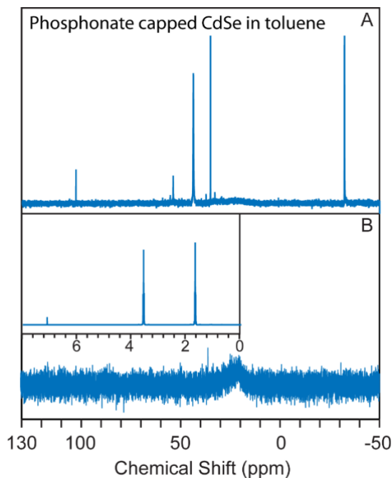
Fig. 3. GPC in situ change of solvent with TDPA-capped CdSe NCs. (A) 31 P NMR of the as-synthesized TDPA-capped CdSe NCs in toluene; (B) 31 P NMR of the sample after traveling through the THF column revealing the purification of the NCs; The inset shows the 1 H NMR of the solvent eluted out with the purified NCs in CDCl 3 , which confirms that the solvent has been changed from toluene to THF.
