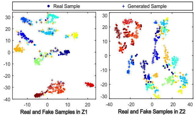
Figure 5. t-SNE [27] visualization results of the real and the generated test sample representations in Z_1 and Z_2 respectively. The solid circles and the cross marks indicate the real and generated representations, and different colors denote different action categories. We observe that real and generated representations which belong to the same category are close to each other. It illustrates that the generative model is capable to “recover” one view conditioned on the other view. And it further demonstrates the effectiveness of the generative strategy in this multi-view scenario.
