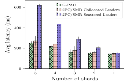
Figure 6: Commit latency vs. number of shards.
