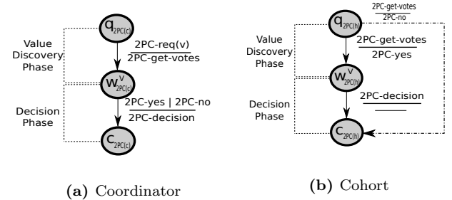
Figure 1: State machine representation of 2PC.
