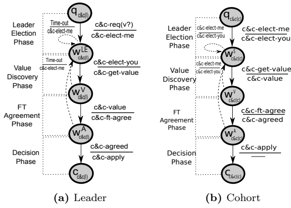
Figure 4: State machines of the C&C framework.
