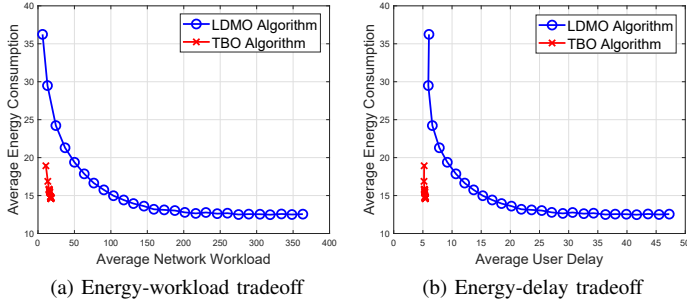
Fig. 2: Comparison between TBO and LDMO algorithms
