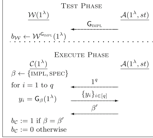
Fig. 13. Stego-freeness game for randomness generation
