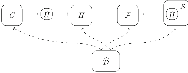
Fig. 12. H -crooked Indifferentiability: distinguisher \widehat{\mathcal{D}} , in the first phase, manufactures and publishes a subverted implementation denoted by \tilde{H} , for ideal primitive H ; then in the second phase, a random string r is published; after that, in the third phase, algorithm C , and simulator \mathcal{S} are developed; the H -crooked-distinguisher \widehat{\mathcal{D}} , in the last phase, either interacting with algorithm C and ideal primitive H , or with ideal primitive \mathcal{F} and simulator \mathcal{S} , returns a decision bit. Here, algorithm C has oracle accesses to \tilde{H} , while simulator \mathcal{S} has oracle accesses to \mathcal{F} and \tilde{H} .
