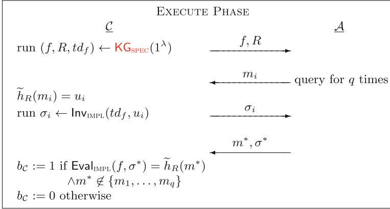
Fig. 6. Game-1: Honest key generation
