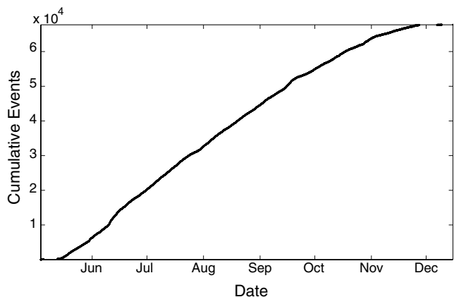
Figure 8. Seismicity rate during the experiment. The cumulative number of events is plotted versus time (month of year, 2013), revealing an essentially constant seismicity rate of \sim 300 per day.
