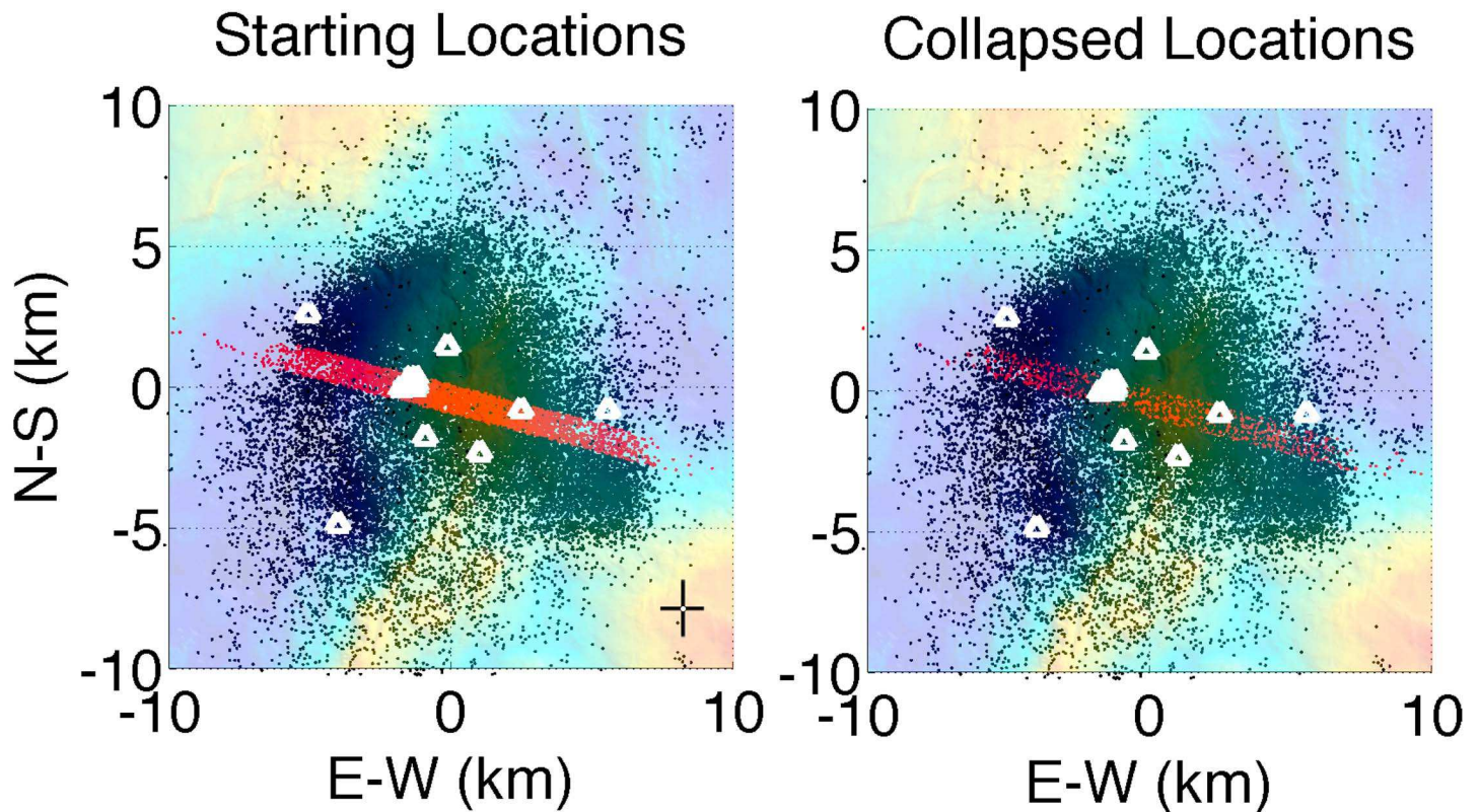
Figure 3. Microearthquake hypocenters with rms errors <200 ms and six or more phase picks across the network. The coordinate system for the axes is centered on the massif ( -33.88792^{\circ}\text{W} , 36.22967^{\circ}\text{N} ). (left) Epicenters from grid search method (black dots) shown on local bathymetry. OBS locations shown with white triangles. Average 1\sigma error bars for the catalog are shown in lower right corner. Events included in cross-section plots in Figure 4 are shown in red. (right) Epicenters after application of collapsing method. Symbols the same as in left panel.
