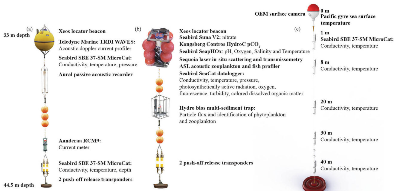
Figure 4. Illustration of the Chukchi Ecosystem Observatory (CEO), including the (a) biophysical, (b) biogeochemical, and (c) freeze-up moorings. Note that the freeze-up mooring includes a surface package, whereas the other two moorings only reach up to 33 m depth. Sensors are calibrated with as many in situ samples as possible. Calibration samples are always collected upon deployment and recovery of the moorings and, depending on other research activity nearby our site, also at other times of the year. p\text{CO}_2 and pH sensors were added in summer 2016.
