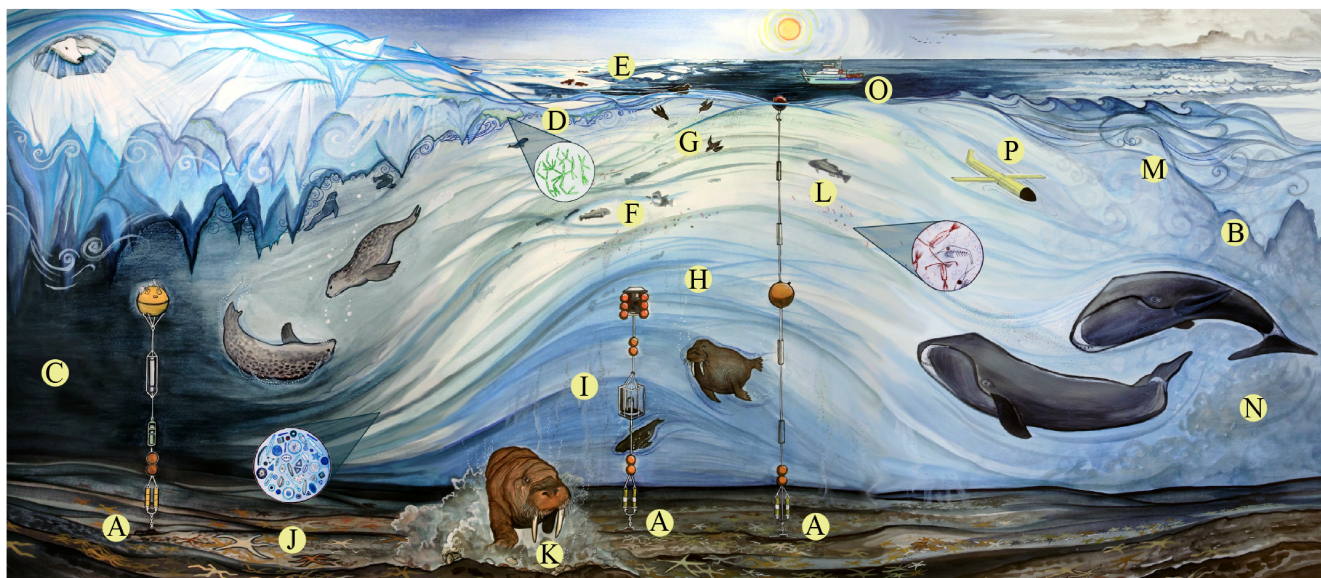
Figure 3. Illustration of the mooring array and the ecosystem at the observatory site. (A) Mooring array, (B) brine rejection, (C) dark winter, (D) sea ice algae bloom, (E) receding sea ice, (F) phytoplankton bloom, (G) stratification, (H) vertical gradient of nutrients and inorganic carbon, (I) sinking particulate organic matter, (J) rich benthic ecosystem, (K) foraging walrus, (L) Arctic cod, (M) storm-induced mixing, (N) senescent planktonic ecosystem, (O) Research Vessel Sikuliaq , and (P) glider. The illustration was painted by Klara Maisch. A high-resolution version can be downloaded from her personal website at https://klaramaisch.com/chukchi-sea-mooring-illustration (last access: 9 November 2018). Examples of walrus and bearded seal sounds are available at http://mather.sfos.uaf.edu/~seth/CEO/Sounds.html (last access: 9 November 2018). A movie describing the observatory in more detail is available at https://www.youtube.com/watch?v=ypmzTuAQ98k&feature=youtu.be (last access: 9 November 2018).
