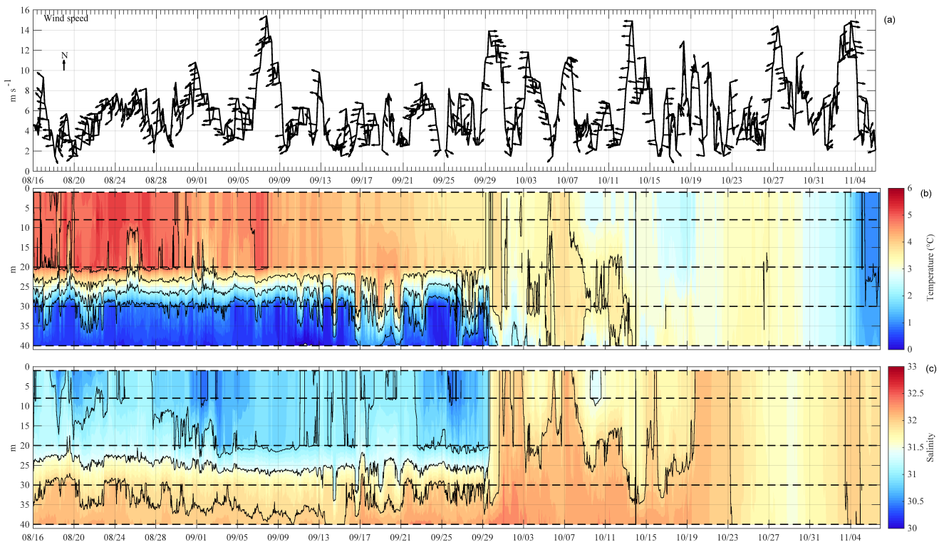
Figure 5. Time series from the NOAA-operated Wiley Post-Will Rogers Memorial Airport weather station and the Chukchi Ecosystem Observatory freeze-up detection mooring deployment in 2015. Shown are (a) wind speed and direction (arrows pointing downwind), (b) temperature ( ^{\circ}\text{C} ), and (c) salinity. Conductivity and temperature sensors were moored at 8, 20, 30, and 40 m (dashed lines) from early September until close to freeze-up at the beginning of November.
