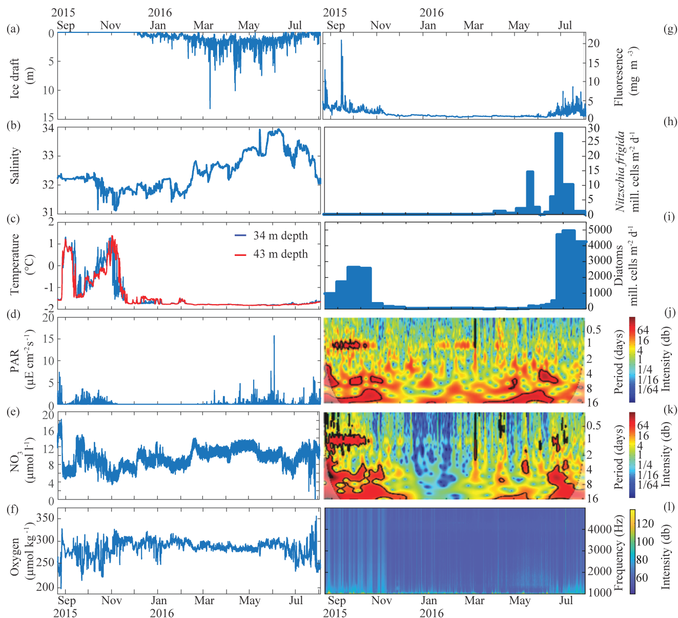
Figure 6. Data from the 2015/16 deployment. Shown are (a) ice draft (m), (b) salinity, (c) temperature ( ^{\circ}\text{C} ), (d) photosynthetically active radiation (PAR, \mu\text{E cm}^{-2} \text{s}^{-1} ), (e) nitrate ( \text{NO}_3 , \mu\text{mol L}^{-1} ), (f) oxygen ( \text{O}_2 , \mu\text{mol kg}^{-1} ), (g) fluorescence ( \text{mg m}^{-3} ), Nitzschia frigida flux (million cells \text{m}^{-2} \text{d}^{-1} ), (i) diatoms (million cells \text{m}^{-2} \text{d}^{-1} ), (j) acoustic zooplankton fish profiler (AZFP, days) 125 KHz, (k) AZFP 38 KHz (days), and (l) acoustic spectra (Hz). In situ \text{NO}_3 water samples were collected at times of the CEO deployment and recovery and were analyzed with standard wet chemical determinations of nitrate + nitrite of frozen samples at the Chesapeake Biological Laboratory. Using the calibration samples as anchor points, a drift of 12 \mu\text{mol L}^{-1} throughout the deployment was found and corrected by linearly detrending the data.
