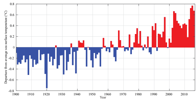
Figure 1. Chukchi Sea continental shelf ( 64 to 74^{\circ}\text{N} and 180 to 157^{\circ}\text{W} ) annual sea surface temperature anomaly over the 1900–2016 period of record from the extended reconstructed sea surface temperature (SST) dataset (Smith et al., 2008). The data are publicly available here: https://www.ncdc.noaa.gov/data-access/marineocean-data/extended-reconstructed-sea-surface-temperature-ersst-v5 (last access: 9 November 2018). Blue bars indicate colder than average temperatures for the given year, whereas red bars indicate warmer than average temperatures. The annual anomalies were computed by subtracting the long-term mean ( 0.114^{\circ}\text{C} ).
