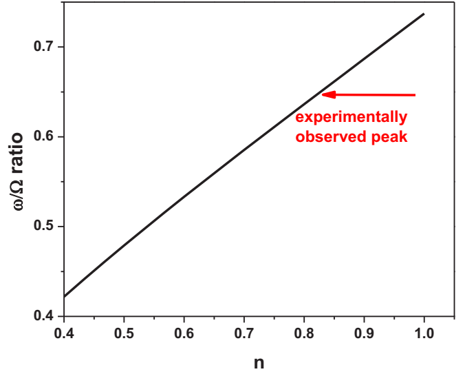
FIG. 1. Ratio of the plasmon-phonon and the phonon frequencies calculated as a function of metal volume fraction n in the Al-Al 2 O 3 metamaterial using Eq. (9). The arrow indicates the frequency of an additional peak observed in the neutron scattering experiment.
