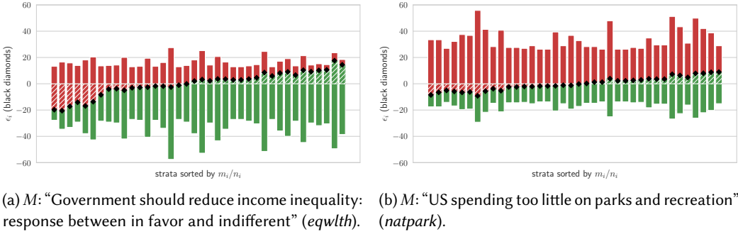
Fig. 8. Distribution of different M over manual 2016 stratification. Overall height of bars is strata size n_i , height of green part (lower end to diamond) is m_i . Position of black diamonds corresponds to \epsilon_i .
