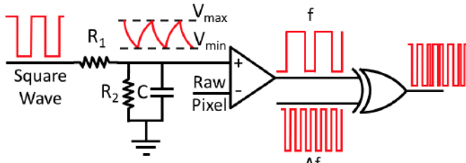
Fig. 7: Pulse Width Modulation Backscatter Architecture.
