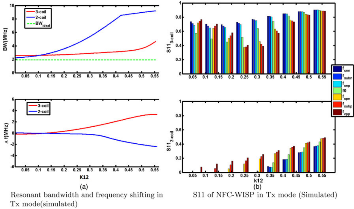
Fig. 5. (a) is the bandwidth performance (includes antenna parasitics and detuned L_2 ; BW_{ideal} refers to minimum bandwidth required by NFC protocol; the BW refers to the bandwidth of highest PDL (even when two resonant frequency appears) at resonant frequency, the resonant frequency normally shifts away from the NFC frequency as k_{12} increases; \Delta f is the frequency offset of the highest resonant frequency to 13.56 MHz. In the NFC-WISP system, it is around 0–0.4. (b) is the S_{11} of NFC load modulation spectrum, f_0 = 13.56\text{MHz} , f_{sub} = 847.5\text{KHz} , f_{data} = 105.9\text{KHz} , f_{subn} = f_0 - f_{sub} , f_{subp} = f_0 + f_{sub} , f_{cnn} = f_{subn} - f_{data} , f_{cnp} = f_{subn} + f_{data} , f_{cpn} = f_{subp} - f_{data} , f_{cpp} = f_{subp} + f_{data} . ( k_{12} refers to the Tx-to-First Rx coil in all systems).
