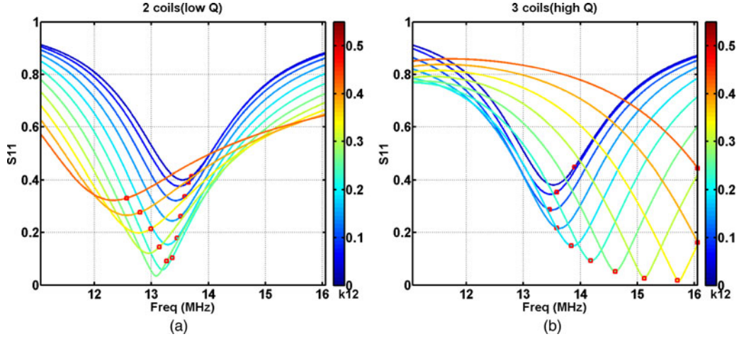
Fig. 6. Simulated S_{11} of the 2-coil and the 3-coil systems in Tx mode (when R_L = R_{L_{Tx}} ) by sweeping transmitted frequency (x-axis); red square marks the resonant frequency where the PDL is maximum, the color of each plot refers to the simulation result with different k .
