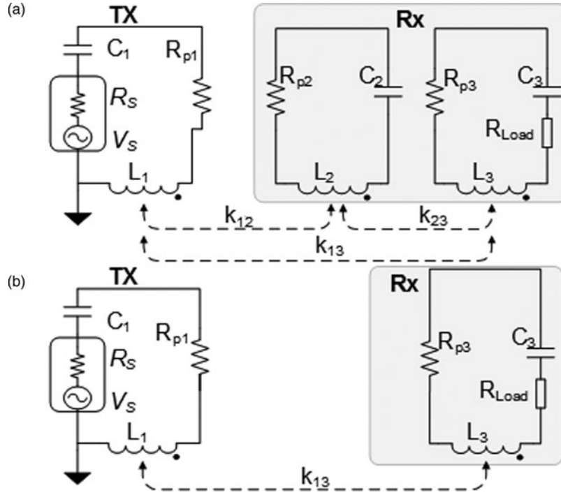
Fig. 3. Block diagram of the NFC wireless power system: (a),(b) refer to 3-coil and 2-coil systems respectively. Tx is the NFC reader and Rx is the NFC tag. R_{pi} and C_i are the equivalent resistance and tuning capacitance of the coil i with inductance of L_i . R_s and R_{load} are the source resistance of NFC reader and the equivalent resistance of the loaded hardware on the NFC tag. k_{ij} is the coupling coefficient between coil i and coil j .
