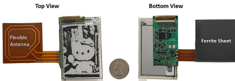
Fig. 1. Prototype of new battery-free NFC-WISP with flexible switchable receiver antenna and 2.7" E-ink display.
