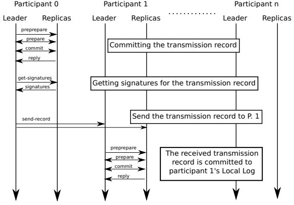
(b) The communication needed to communicate a message from participant 0 to participant 1 where send and receive instructions are involved
