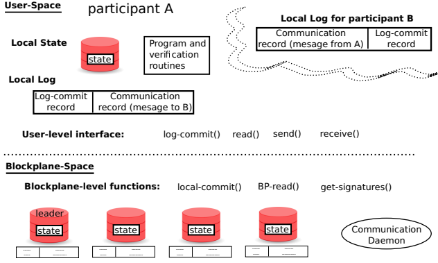
Fig. 1. An illustration of a Blockplane deployment in participant A distinguishing between user-space and Blockplane-space and showing an example of Local Logs in a scenario with two participants. Each log contains log-commit and communication records.
