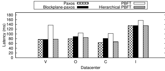
Fig. 7. The performance of Blockplane-paxos in comparison with paxos, PBFT, and Hierarchical PBFT.
