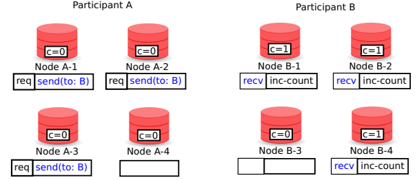
Fig. 2. An example of the state of Blockplane nodes.
