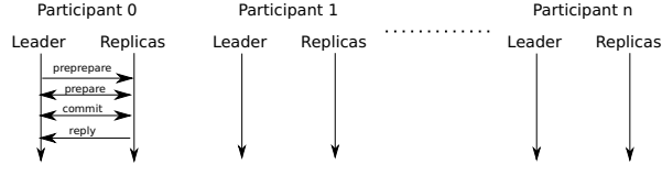
(a) The communication needed to commit a value using local-commit in participant 0
