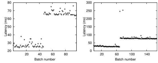
Fig. 8. The performance of reacting to two types of node failures (a) Backup failure (b) Primary failure
