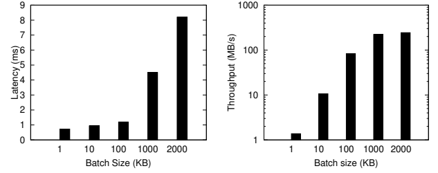
Fig. 4. The performance of local commitment while varying the block size
