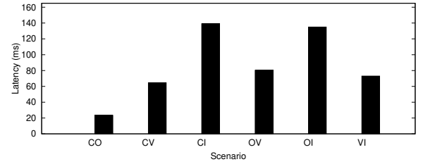
Fig. 6. The performance of communication between participants
