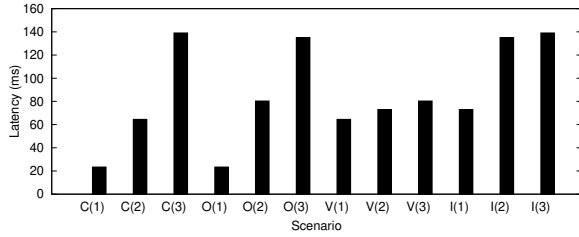
Fig. 5. The performance of committing with geo-correlated byzantine fault-tolerance
