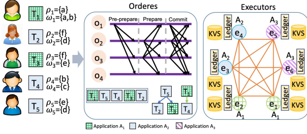
Fig. 2. The Components of OXII Paradigm
