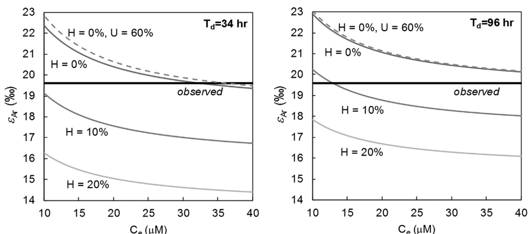
Fig. 4. Sensitivity of the N. maritimus numerical model (Fig. 1b) to HCO_3^- import and incorporation of respiratory CO_2 (including from urea metabolism). Solid lines show HCO_3^- ( H ) import equivalent to 0, 10, or 20% of total carbon fixation ( fix ); dashed lines show incorporation of respiratory CO_2 ( U , urea) at 60% of fix . Endmember values of \delta_{He} and \delta_U were +1\text{‰} and -23\text{‰} , respectively. A slow generation time ( T_d = 96 h) moderately diminishes the effects of the H and U fluxes. The intersection of the observed \varepsilon_{Ar} and the H = 0\% curves at > 30 \mu M C_e and a 34-h doubling time ( T_d ) reflects the behavior of the low-pH cultures of Könneke et al. (2012), while the 96-h doubling time reflects the observations from marine POM (Hurley et al., 2019).
