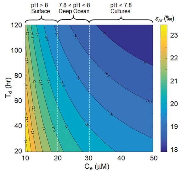
Fig. 3. Predicted response of \epsilon_{Ar} to [CO 2(aq) ] and \mu (expressed as doubling time, T_d ) for N. maritimus . The enzymatic parameters that affect these results currently are based on assumptions (Table 1), with values optimized to reproduce existing \delta^{13}\text{C} data for N. maritimus (Könneke et al., 2012), for marine Thaumarchaeota more generally (Schouten et al., 2013; Pearson et al., 2016), and to agree with an existing data set for marine POM (Hurley et al., 2019).
