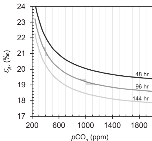
Fig. 5. Predicted sensitivity of the \epsilon_{Ar} proxy to changes in atmospheric pCO_2 and three different doubling times ( T_d ) for archaeal growth. Curves are calculated based on 15 °C seawater, pH 8.0, a temperature-sensitive Henry's Law constant (Zeebe and Wolf-Gladrow, 2001), and assuming equilibrium partitioning. Shaded areas indicate the uncertainty in reconstructed pCO_2 values that would result from analytical precision of \pm 0.2\% . Most records would be accompanied by errors due to uncertainty in reconstructing \delta_{He} , implying that the shown uncertainties of +200/–100 ppm at 1000-ppm pCO_2 represent the best-case scenario.
