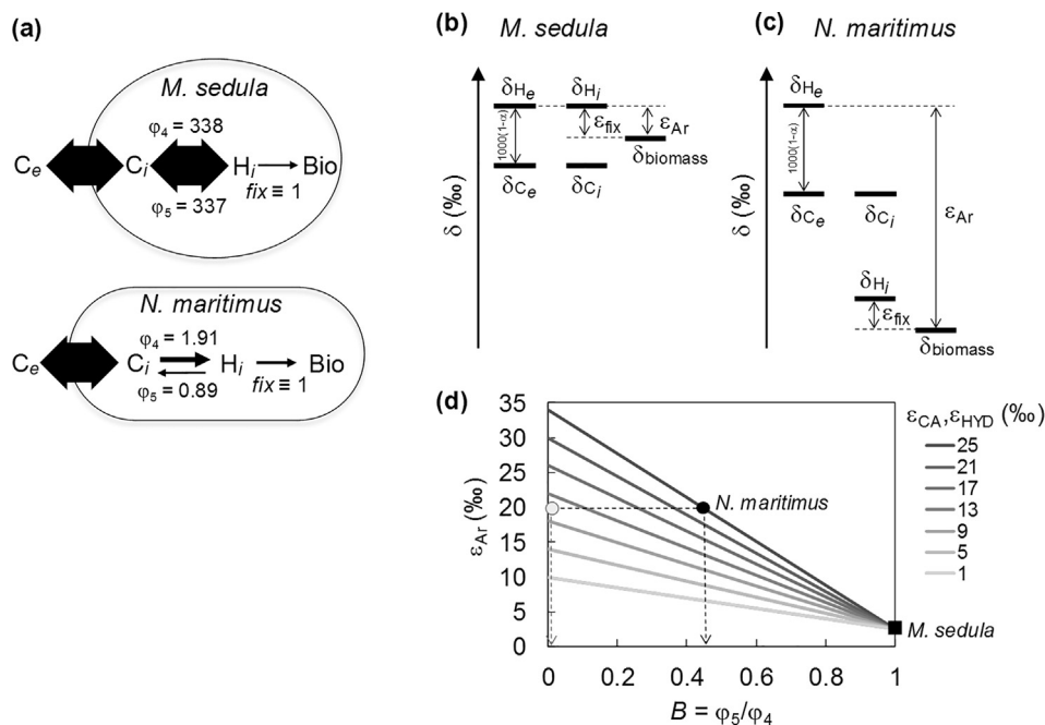
Fig. 2. (a) Solution to the simplified flux-balance model. Widths of arrows highlight the flux magnitudes for intracellular C_i \rightleftharpoons H_i interconversion, normalized to carbon fixation ( \text{fix} , Table 1). (b), (c) Relative \delta^{13}\text{C} values for intracellular and extracellular carbon pools in the M. sedula and N. maritimus simple models (vertical axis not to scale). In both b and c, \varepsilon_{A_r} reflects the difference between \delta_{\text{biomass}} and the external environment ( \delta_{H_e} ). (d) Illustration of the relationship between dehydration ( B = \varphi_5/\varphi_4 ) ratio and \varepsilon_{A_r} . When B approaches 1, as for M. sedula , H_i is in equilibrium and \varepsilon_{A_r} approaches \varepsilon_{\text{fix}} , regardless of the KIE chosen for \varepsilon_{\text{CA}} or \varepsilon_{\text{HYD}} . For N. maritimus , neither \varepsilon_{\text{HYD}} nor B is known uniquely, but the maximum allowed value of B is 0.47 (assuming \varepsilon_{\text{HYD}} is not larger than the assumed 25‰ KIE for abiotic hydration); in the limit of B \rightarrow 0 , \varepsilon_{\text{HYD}} cannot be < 11\% .
