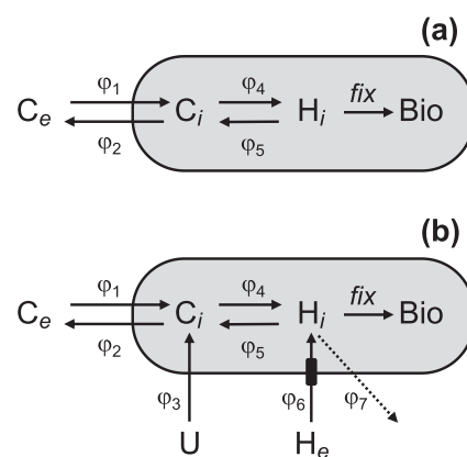
Fig. 1. (a) Simplified analytical and (b) full numerical 3HP/4HB flux-balance models. Carbon pools: C_e , external [\text{CO}_{2(aq)}] ; C_i , internal [\text{CO}_{2(aq)}] ; H_e , external [\text{HCO}_3^-] ; H_i , internal [\text{HCO}_3^-] ; U, urea or other LMW organic metabolites metabolized to \text{CO}_2 ; Bio, total cell biomass. Fluxes: \varphi_1 , diffusion of \text{CO}_2 into the cell; \varphi_2 , diffusion of \text{CO}_2 out of the cell; \varphi_3 , \text{CO}_2 derived from metabolism of organic substances; \varphi_4 , hydration of \text{CO}_2 \rightarrow \text{HCO}_3^- ; \varphi_5 , dehydration of \text{HCO}_3^- \rightarrow \text{CO}_2 ; \varphi_6 , active import of \text{HCO}_3^- ; \varphi_7 , diffusive leakage of \text{HCO}_3^- (as \text{H}_2\text{CO}_3 ; Mangan et al., 2016); \text{fix} , autotrophic carbon fixation rate. N. maritimus is rod-shaped, while M. sedula is coccoid. The simplified version assumes \varphi_3 , \varphi_6 , and \varphi_7 are zero.
