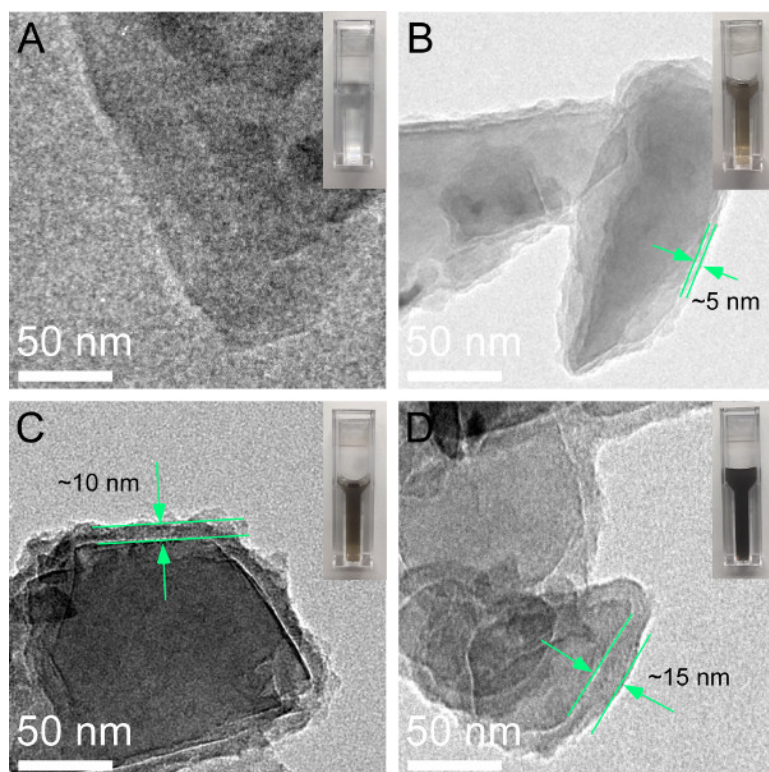
Figure 1. Characterization of the thicknesses of PDA layers on the surfaces of 100 nm NDs with varied concentrations of DA (0, 50, 75, and 100 \mu\text{g}/\text{mL} ) and their corresponding TEM images. The average thicknesses of each PDA layer are \sim 5 nm ( B ), \sim 10 nm ( C ), and \sim 15 nm ( D ), respectively. The inset photograph shows the colorimetric change in the corresponding samples. Please click here to view a larger version of this figure.
