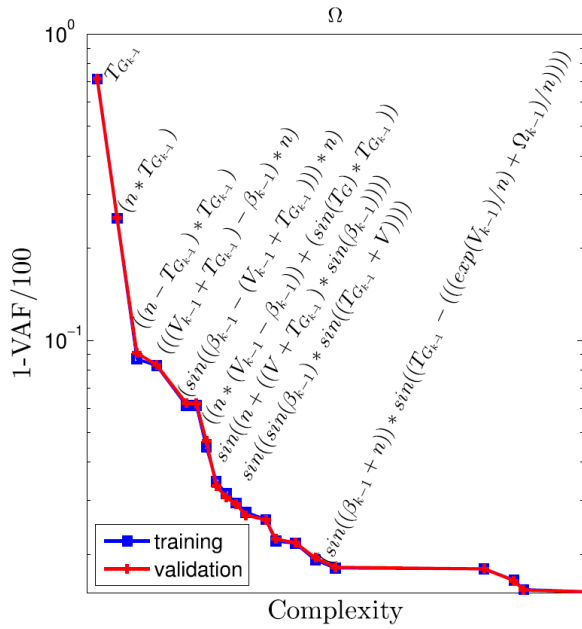
FIG. 4. Example Pareto front showing trade-off between solution complexity and variance accounted for (VAF). Reproduced with permission from La Cava et al. 50
