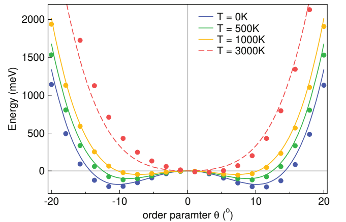
FIG. 6. Landau free energy G for perovskite \text{LaNiO}_3 as a function of the order parameter \theta at different temperatures. Both solid and dashed lines are calculated using Equation 1 with coefficients reported in Ref. 82. Only solid lines are used during the training. The filled symbols correspond to GPSR predicted results using Equation 2.
