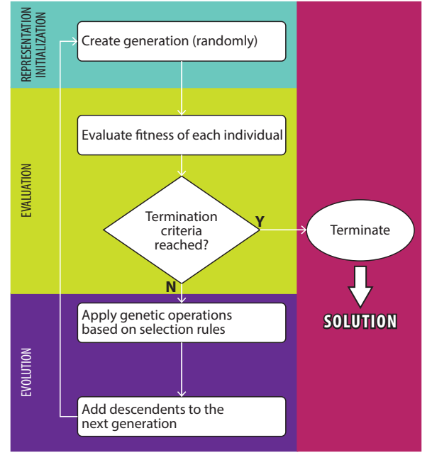
FIG. 3. Genetic programming flowchart depicting the iterative solution-finding process.
