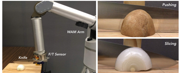
Fig. 6. Experiment setup.
