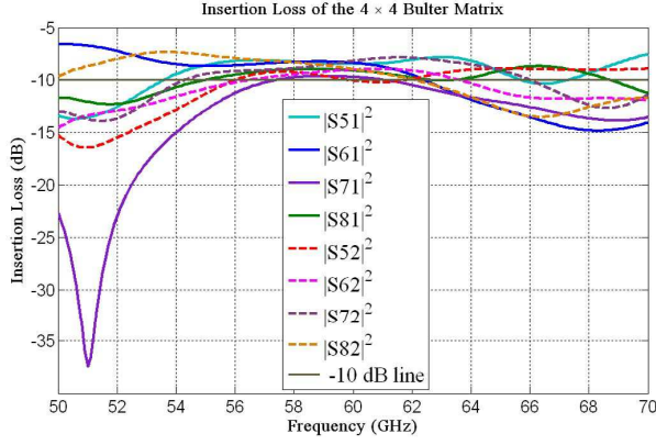
Fig. 4. Simulated maximum output magnitude unbalance is less than \pm 1.2 dB
