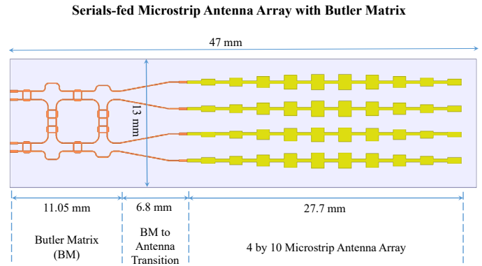
Fig. 1. Outline dimensions of the proposed antenna system
