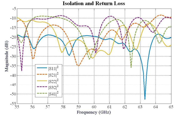
Fig. 10. Simulated port isolation and return loss of proposed antenna system
