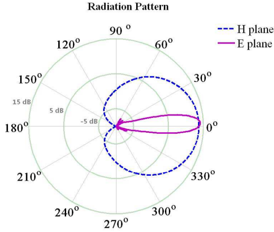
Fig. 8. Gain of a Single 1 \times 10 patch array
