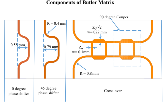
Fig. 2. Critical Dimensions of Butler Matrix Components
