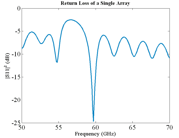
Fig. 7. Return Loss of a Single 1 \times 10 patch array shows the -10dB BW of the antenna array is 1GHz
