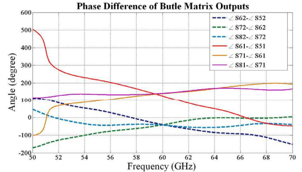
Fig. 3. Simulated BM phase increments v.s frequency. Maximum phase unbalance is less than \pm 7^\circ
