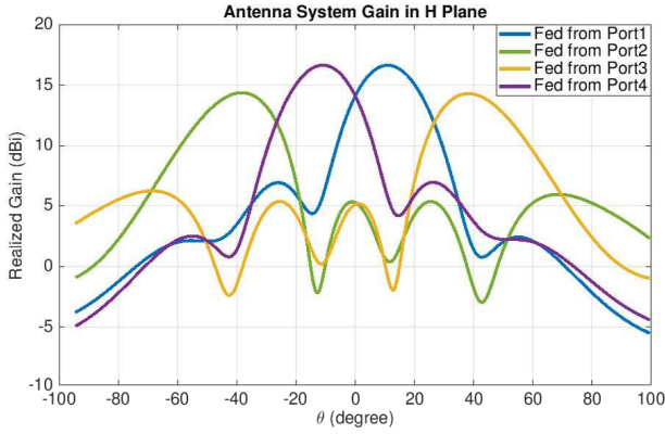
Fig. 9. Realized Gain of Antenna System
