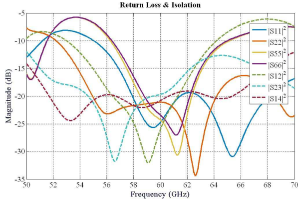
Fig. 5. Simulated return loss and port isolation of Butler Matrix
