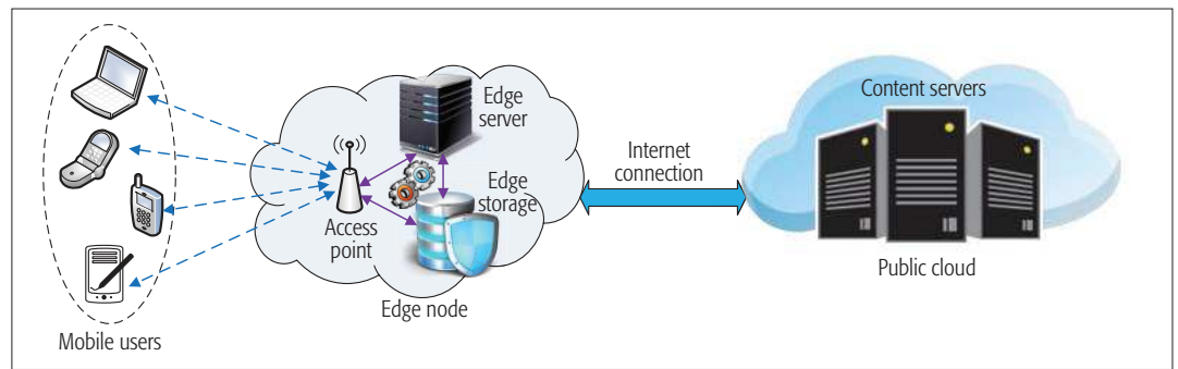
FIGURE 1. A general architecture of a mobile edge caching network.
