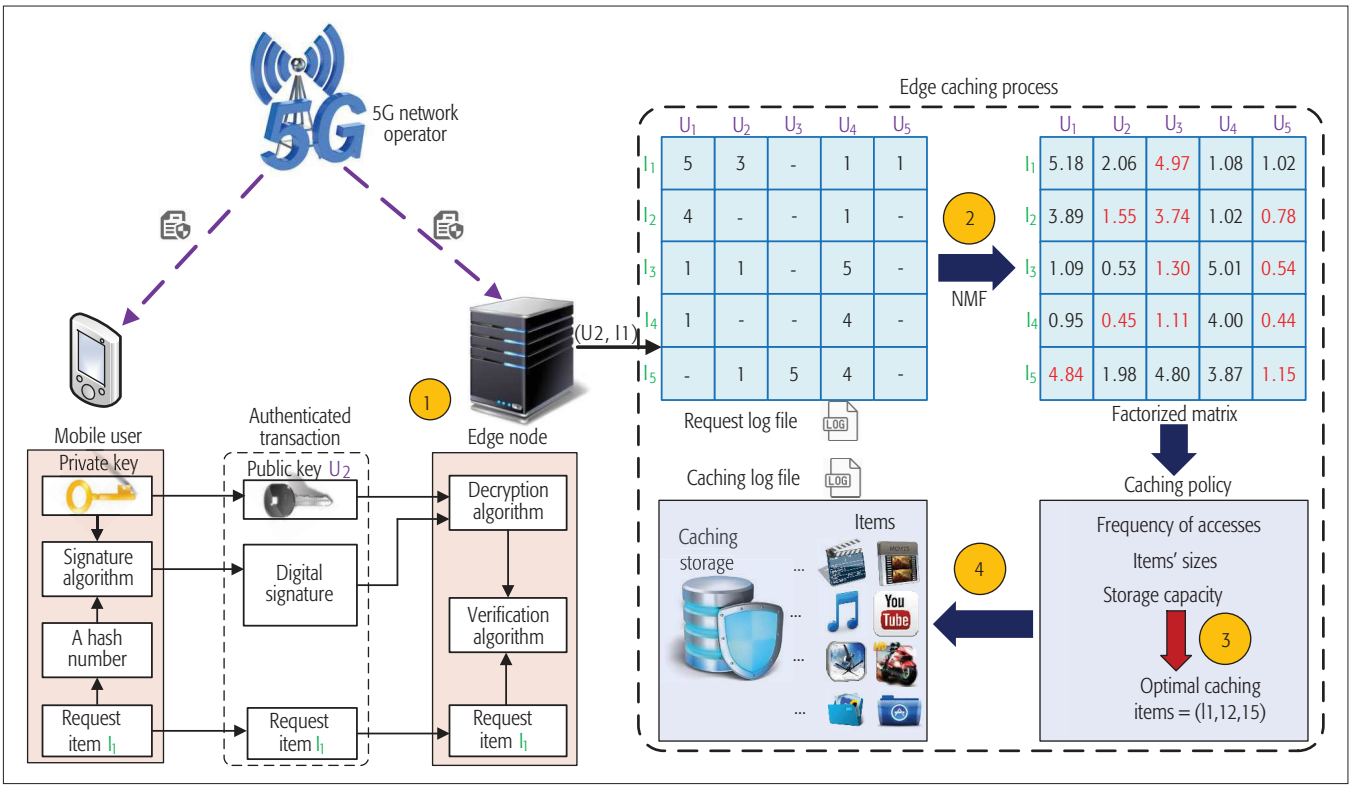
FIGURE 2. An illustration of the proposed smart caching system.
