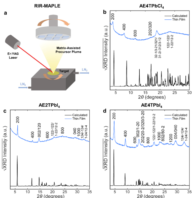
Figure 2. Schematic of the RIR-MAPLE process (a), and Cu K \alpha XRD patterns of oligothiophene perovskite films deposited by RIR-MAPLE, referenced against patterns calculated using computationally optimized structures from van der Waals corrected semilocal DFT: (b) \text{AE4TPbCl}_4 , (c) \text{AE2TPbI}_4 and (d) \text{AE4TPbI}_4 . Comparison of the film XRD patterns against the calculated patterns indicates that all of the peaks in the former may be assigned to Miller indices corresponding to reasonably prominent peaks in the latter. Similar sets of reflections (e.g., h00 , 0k0 , 122 ) appear in the patterns of both ( \text{AE2T}/\text{AE4T} ) \text{PbI}_4 , indicating similar texture in these closely related materials. The \text{AE4TPbCl}_4 pattern contains fewer and less-well-defined peaks. However, features resembling those in the other patterns are evident, such as the first three h00 reflections, which decrease in intensity in a manner consistent with the predicted pattern and the other two perovskites. The theory-derived \text{AE4TPbCl}_4 pattern slightly underestimates the lattice constant along the a axis; however, the inferred values are still broadly consistent with the expected structure. Note that another recent computational study on \text{AE4TPbCl}_4 predicts a similar value for the interlayer lattice parameter as our DFT calculations; 2 however, also note that relatively subtle changes in the configuration of the quaterthiophene cations can have substantial impact on the lattice parameters in the DFT-predicted structures, as explored further in the Supporting Information (Figure S2, Table S2). Accurate determination of all subtleties of the structure would require the growth and XRD refinement of single crystals, which is beyond the scope of this work. Importantly, the key optoelectronic properties reported below are experimentally derived and thus not affected by small structural deviations between the computationally assumed model and the experimental material.
