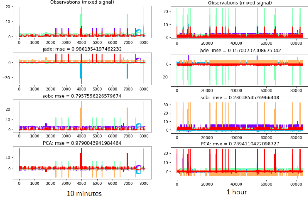
Figure 2: Five application traces [6] were separated with BSS techniques and PCA. Both visual examination and the MSE that the component signals returned by BSS techniques are closely resemble ground truth (note: sign is arbitrary). The PCA signals are much less accurate. Also, while MSE was lowest for a long trace (the y axis represents frequency, and the x axis is time), even the first ten minutes of I/Os led to low MSE for BSS.
