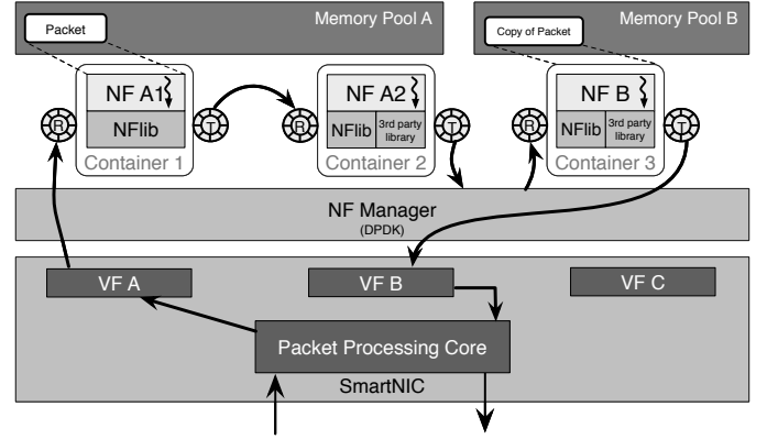
Fig. 3. System Architecture - Memory Isolation and SmartNIC
