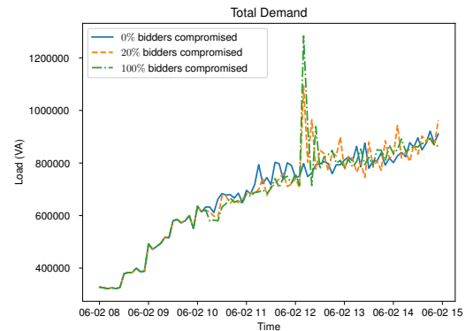
Fig. 10: Demand Peak Created in Attack Scenario 1
