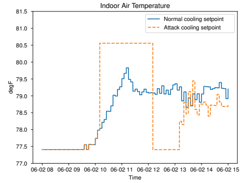
Fig. 9: Indoor Temperature Setpoint of HVAC System
