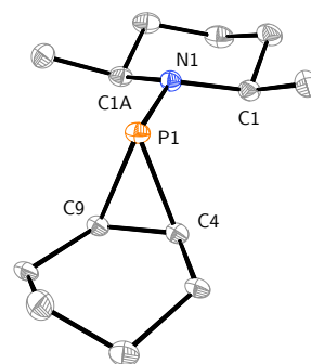
Figure 10 Solid-state molecular structure of anti,cis - Me_2PipPC_6H_{10} with ellipsoids at the 50% probability level. Hydrogen atoms and second domain of the disordered cyclohexane ring are omitted for clarity. Selected interatomic distances (Å) and angles (°): P1–C 1.877 (avg), P1–N1 1.7364(8), C1–N1 1.4794(7); N1–P1–C4 108.5(3), N1–P1–C9 105.0(2), C4–P1–C9 47.21(7), C1–N1–C1A 115.29(7), C1–N1–P1 116.50(4).
