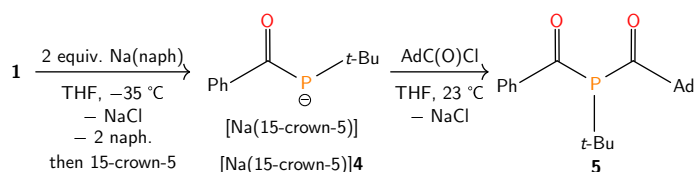
Scheme 2 Synthesis of [Na(15-crown-5)] 4 and 5 .
