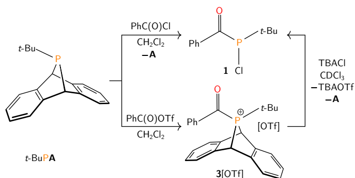
Scheme 1 Synthesis of 1 and 3[OTf] .
